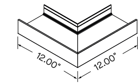
Knife Edge Ceiling-to-Ceiling Outside Corner
