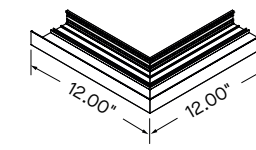
Classic Ceiling-to-Ceiling Inside Corner
