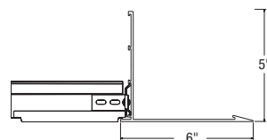
Axiom Knife Edge Profile (AXKE5STR)
