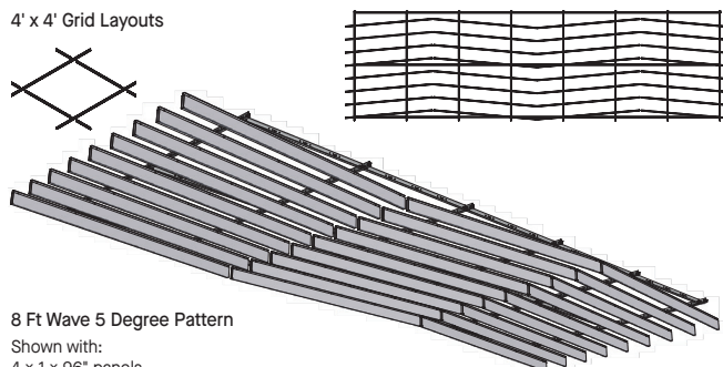
4' x 4' Grid Layouts
