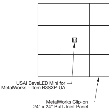
USAI BeveLED for MetalWorks Fixture Housing
