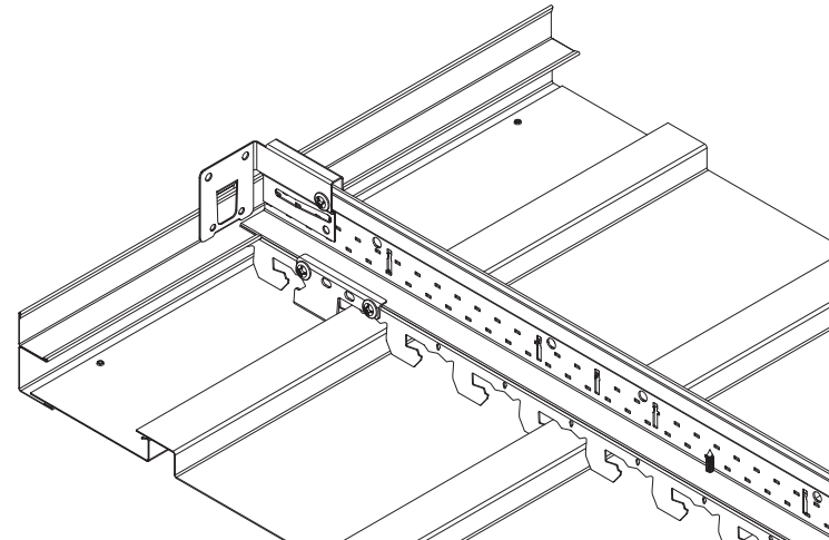
(Fig 39) Attached wall, cut plank retaining hook edge
