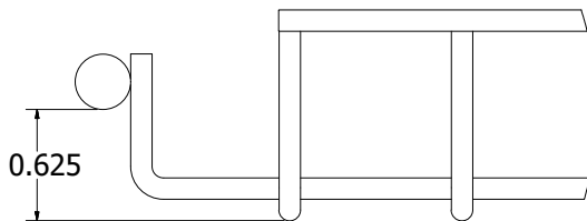
Edge Detail for Welded Tegular
