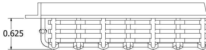
Edge Detail for Woven Tegular
