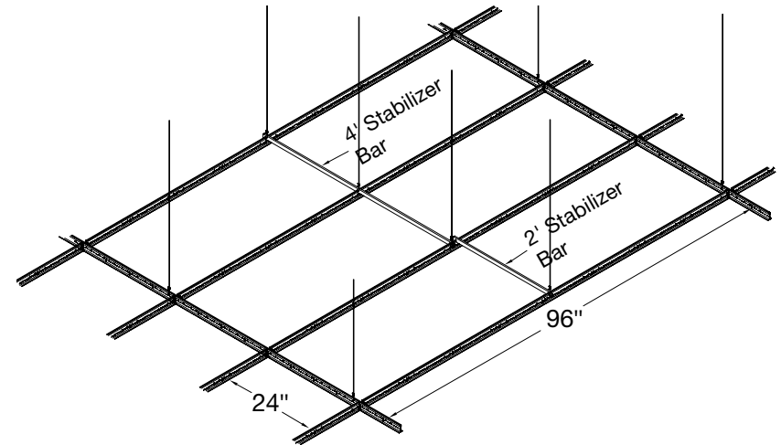
24" x 96" Panel Installation
