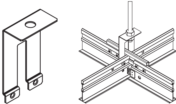
PMHC – Prelude Max Hanging Clip
