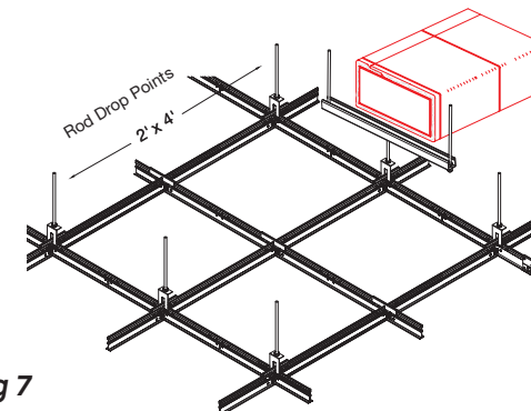
PMHC – Prelude Max Hanging Clip
