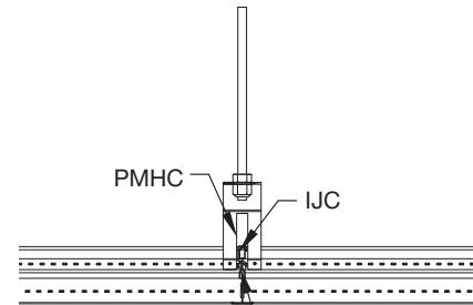
Prelude XL Max 4' Cross Tee
