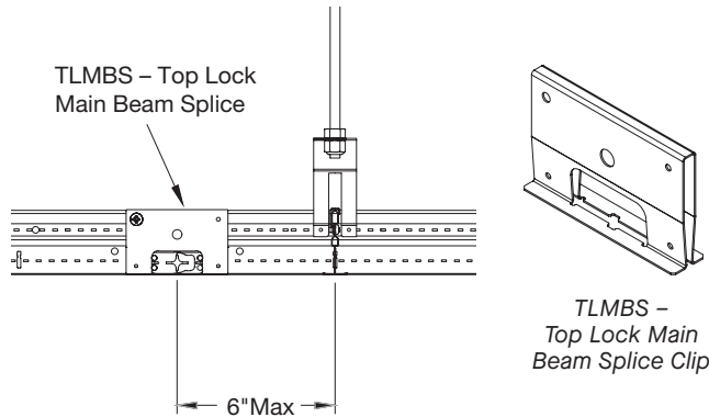
Fig 9 Top Lock Main Beam Splice Clip Installation on two Prelude® XL Max® Main Beams
