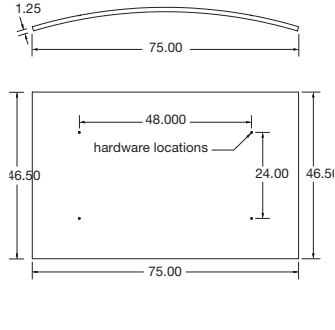
Hill – Hardware side
