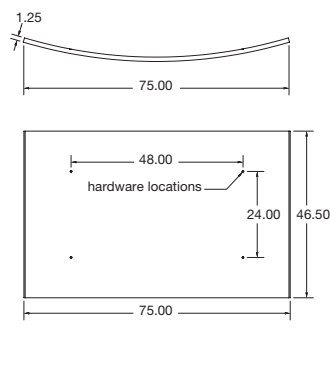
Valley – Hardware side
