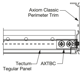
① Discontinuous system using Axiom trim solutions
