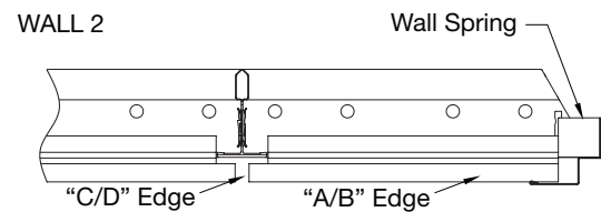
Wall Spring inserted between panel edge and molding. NOTE: Hold Down Clips not shown, but required.
