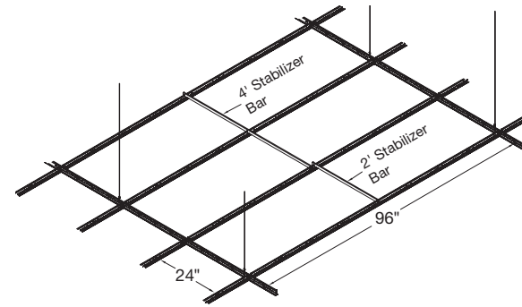
24" x 96" Panel Installation
