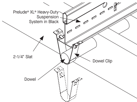
Ceiling Dowel Assembly
