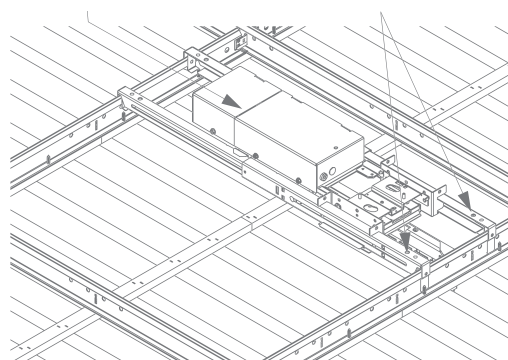
USAI® Micro™ for WOODWORKS – Vertical Slats Fixture Housing USAI Grid Mounting Bars Item UA2
