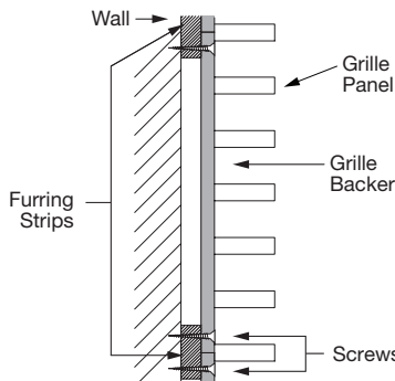
Wall Backer Assembly
