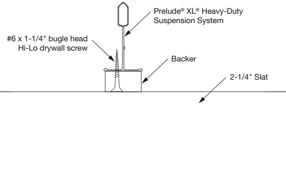
Screw Attachment Detail
