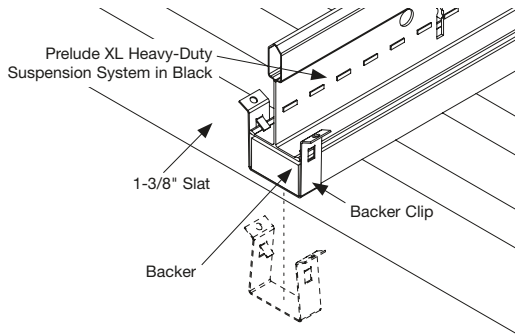
Ceiling Backer Assembly
