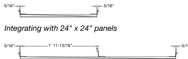
Integrating with 24" x 48" panels
