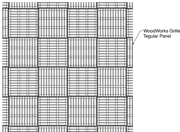
① 6723F51L2T9 Grille Tegular Installation Layout
