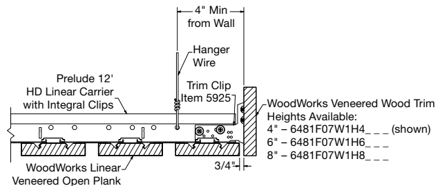
② Linear Veneered Open Perimeter Trim
