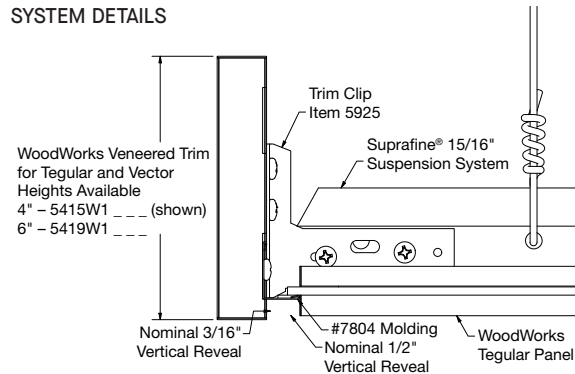
① Tegular Panel Perimeter
