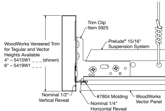
② Vector Panel Perimeter Trim
