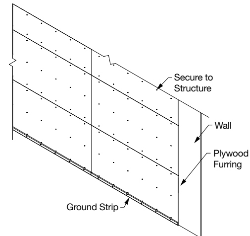
Furring for Vertical/Horizontal Stacking Installation
