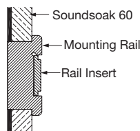
Soundsoak 60 panel with Chair Rail – Mounting Rail with Easel Ledge (field-painted)
