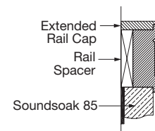
Soundsoak 85 panel with Chair Rail – Mounting Rail with Rail Insert, Extended Rail Cap and Rail Spacer
