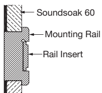
Soundsoak® 60 panel with Chair Rail – Mounting with Rail Insert
