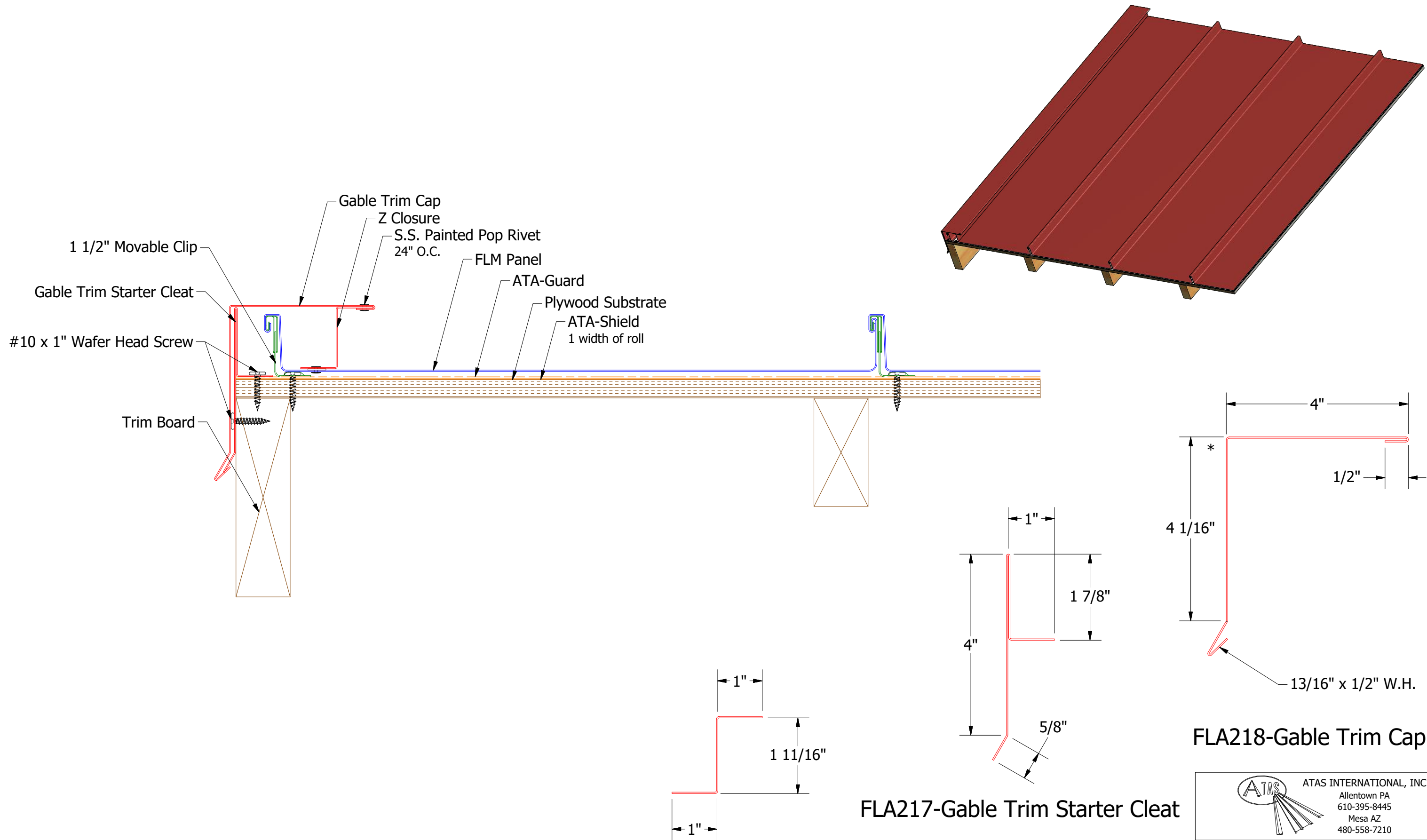
FLA916-Z Closure
