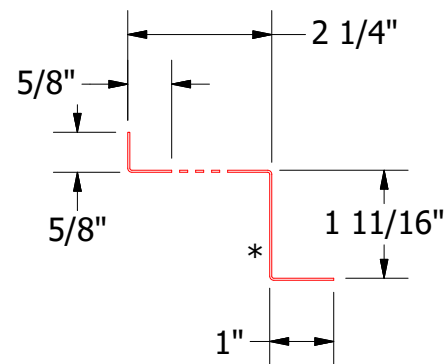
Vented Z Closure
