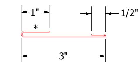
FLA962-Utility Cleat
