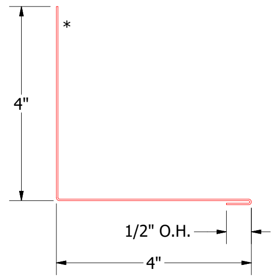
FLA410-Sidewall Trim
