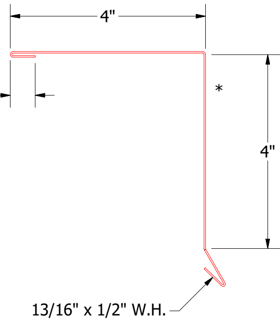
FLA218-Gable Trim Cap
