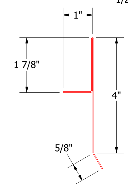
FLA217-Gable Trim Starter Cleat
