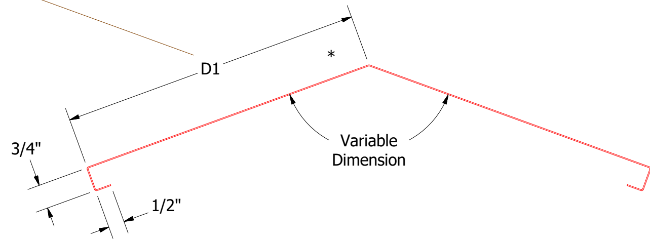
Vented Ridge Cap
