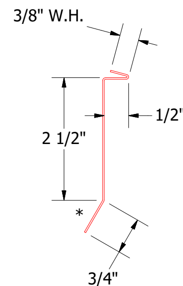
FLA980-Counterflashing
