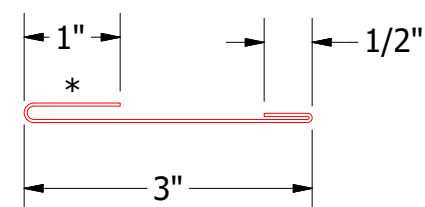
FLA962-Utility Cleat
