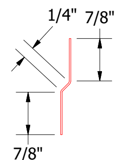
FLA975-Joggle Cleat
