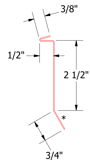
FLA980-Counterflashing
