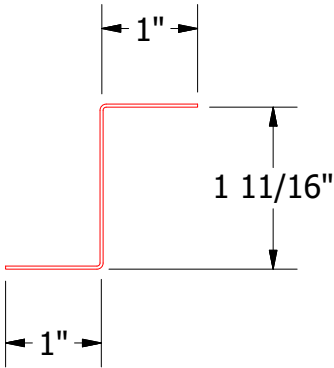
FLA916-Z Closure
