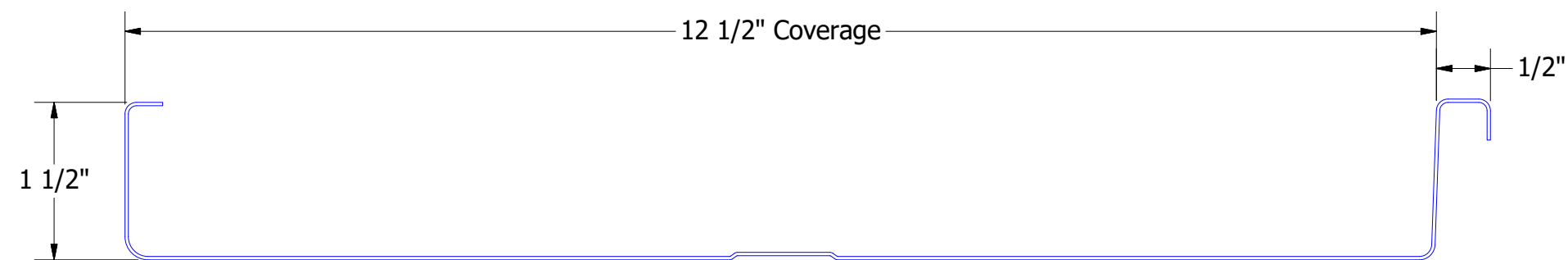
FLM125
