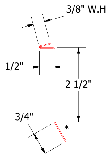
FLA980-Counterflashing
