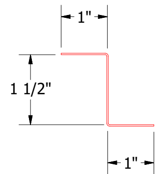
FLA916-Z Closure
