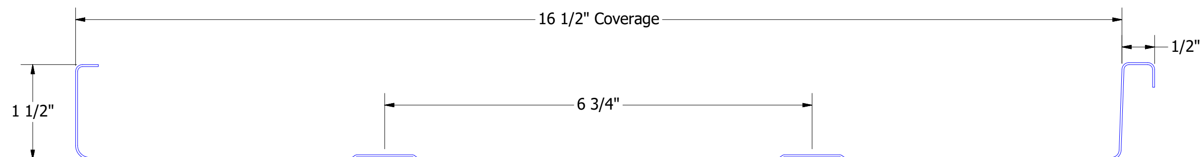
FLM165
