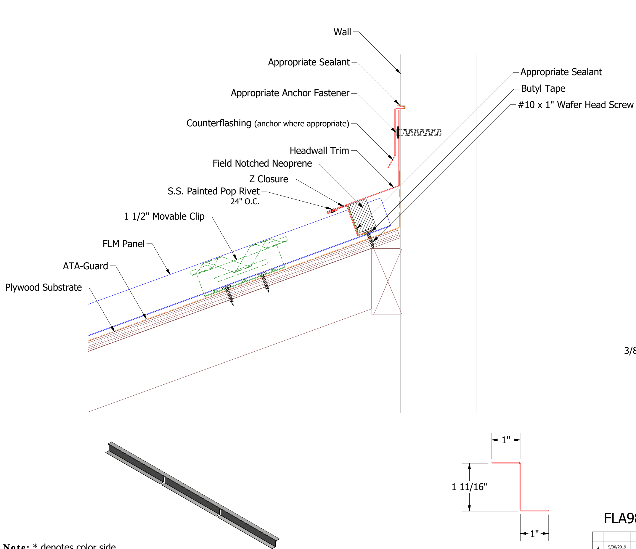
FLA916-Z Closure
