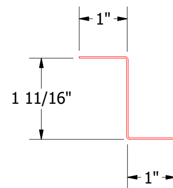
FLA916-Z Closure
