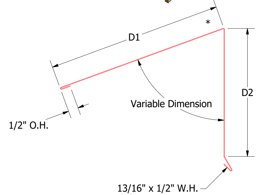
FLA346-Shed Ridge Cap
