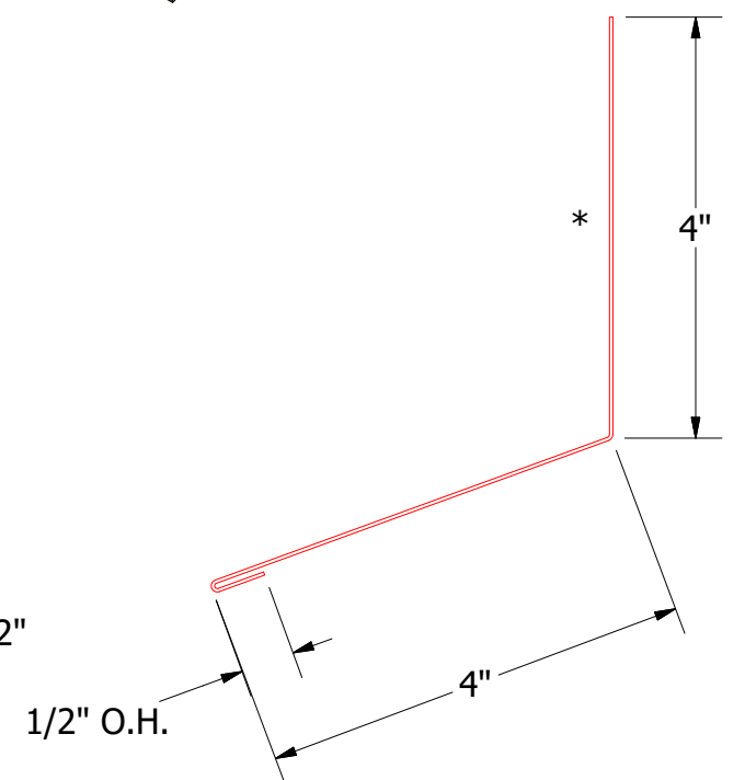
FLA500-Headwall Transition
