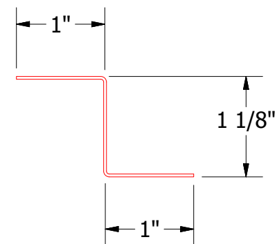
FLA914-Z Closure
