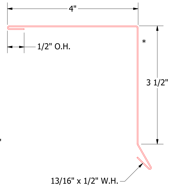
FLA212-Gable Trim Cap
