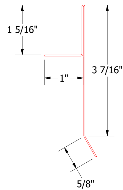
FLA216-Gable Starter Cleat
