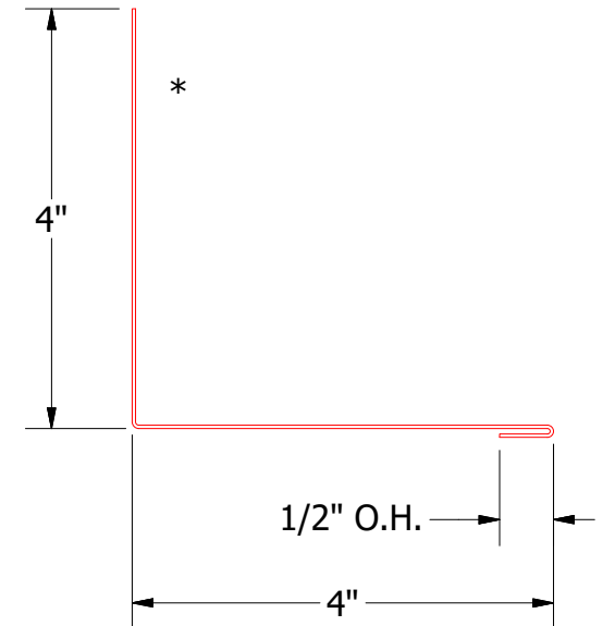
FLA410-Sidewall Trim
