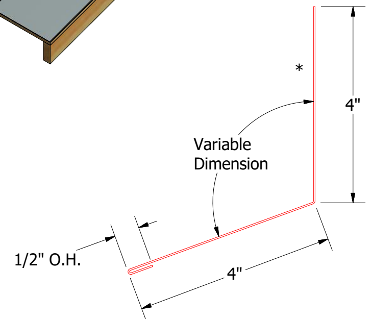
FLA500-Headwall Trim
