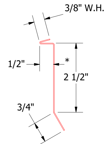
FLA980-Counterflashing
