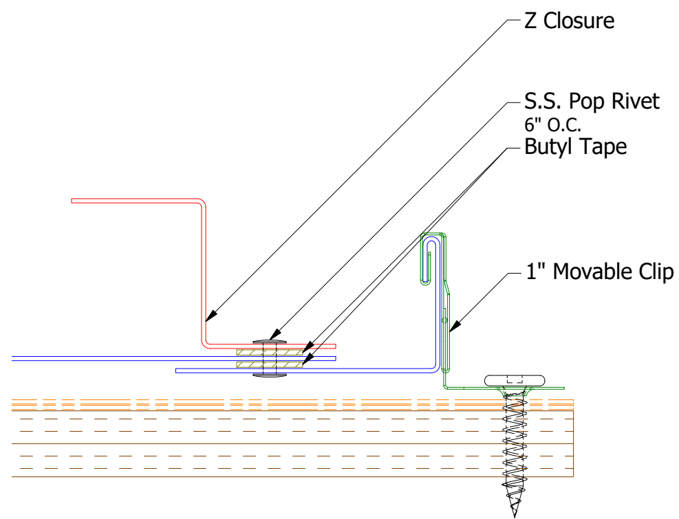
Butyl Tape Detail
