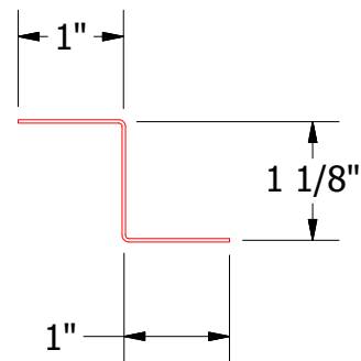
FLA914-Z Closure
