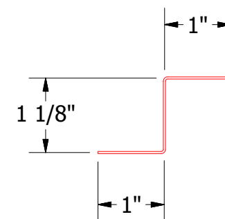
FLA914-Z Closure
