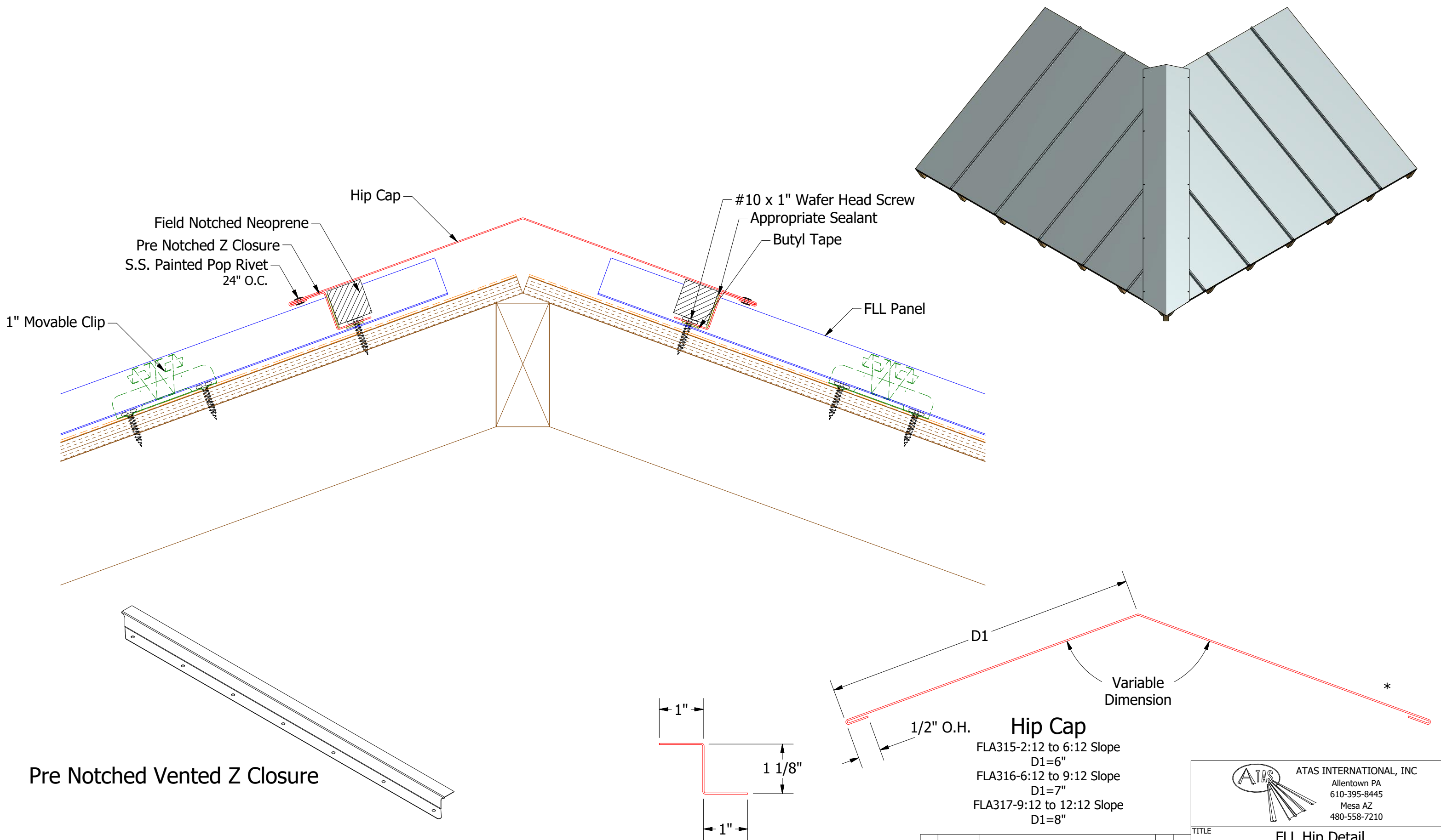
FLA914-Z Closure
