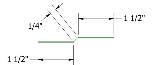
FLA975-Joggle Cleat
