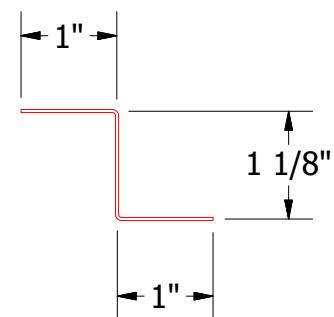
FLA914-Z Closure
