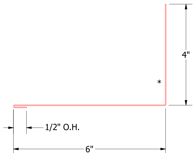
FLA411-Sidewall Trim
