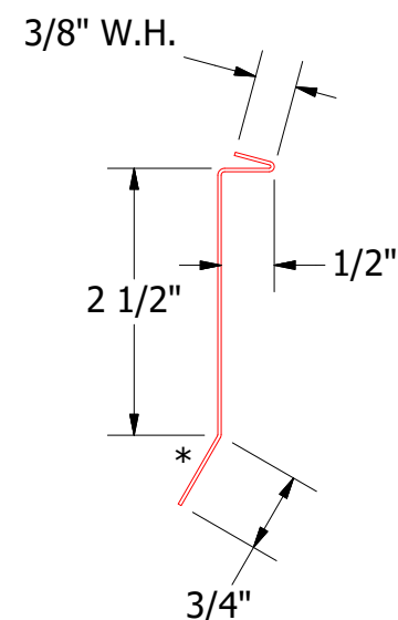
FLA980-Counterflashing
