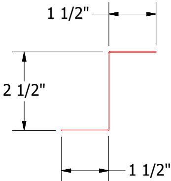
FLA910-Z Closure
