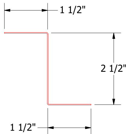
FLA910-Z Closure
