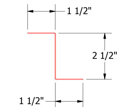
FLA910-Z Closure
