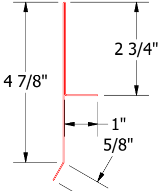
FLA211-Gable Starter Cleat
