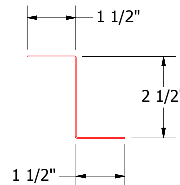
FLA910-Z Closure
