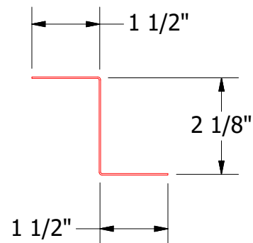
FLA912-Z Closure
