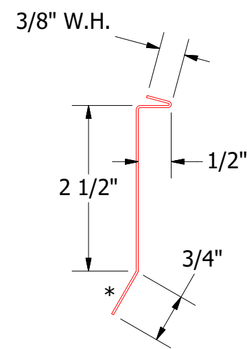
Counterflashing
