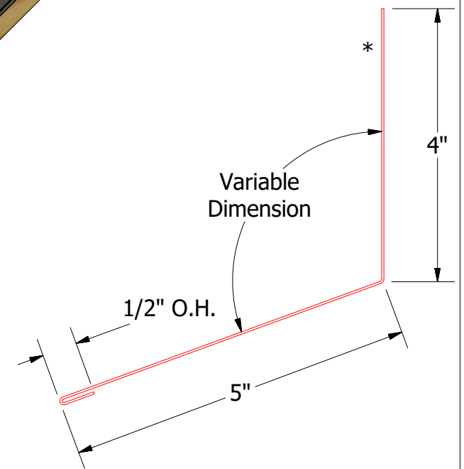
Headwall Trim
