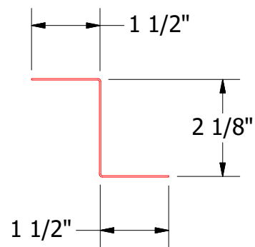
FLA914-Z Closure
