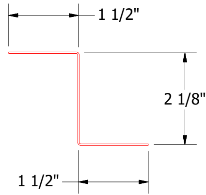
FLA912-Z Closure
