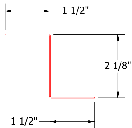
Z Closure
