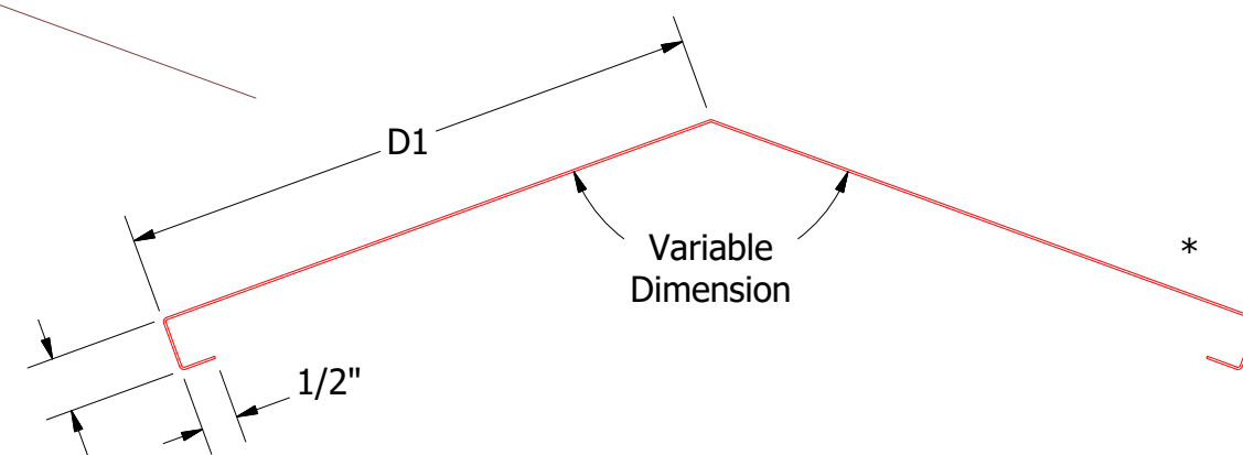
Vented Ridge Cap
