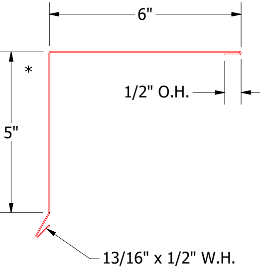
FLA210-Gabe Trim Cap
