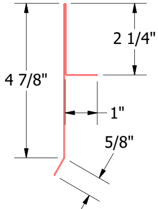
FLA215-Gable Starter Cleat
