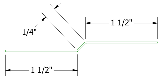
FLA976-Joggle Cleat (NTS)
