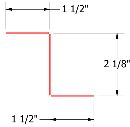
FLA912-Z Closure
