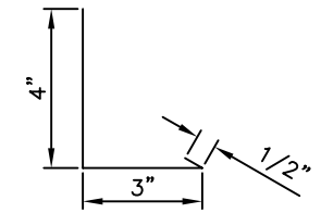
HSA440 STEP FLASHING
