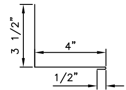
HSA410 SIDEWALL TRIM
