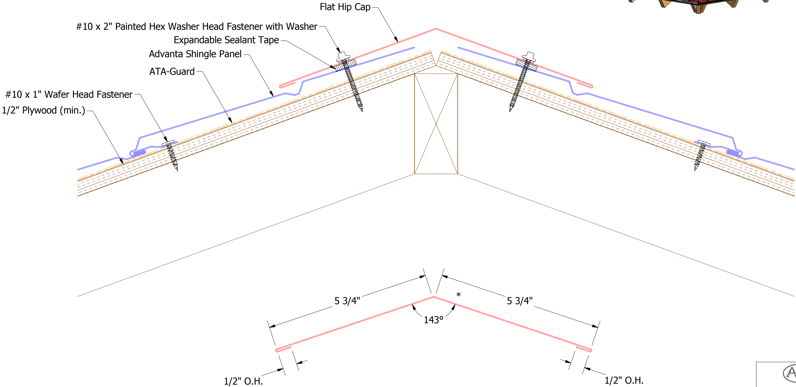
HSA304 - Flat Hip Cap
