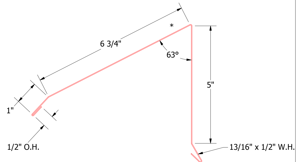
HSA362 - Vented Shed Ridge Cap
