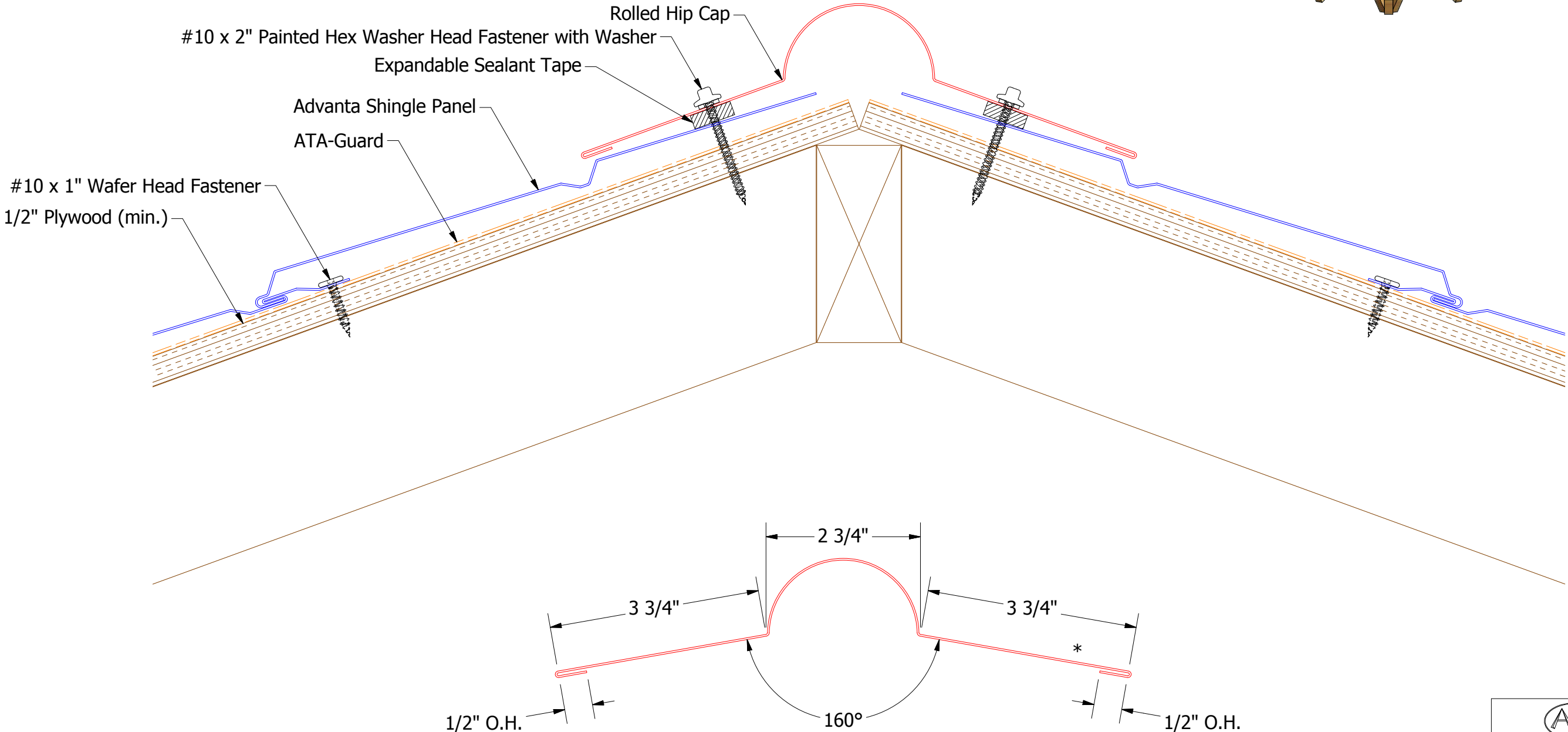
HSA303 - Rolled Hip Cap
