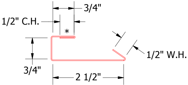
HSA201-Channel Trim
