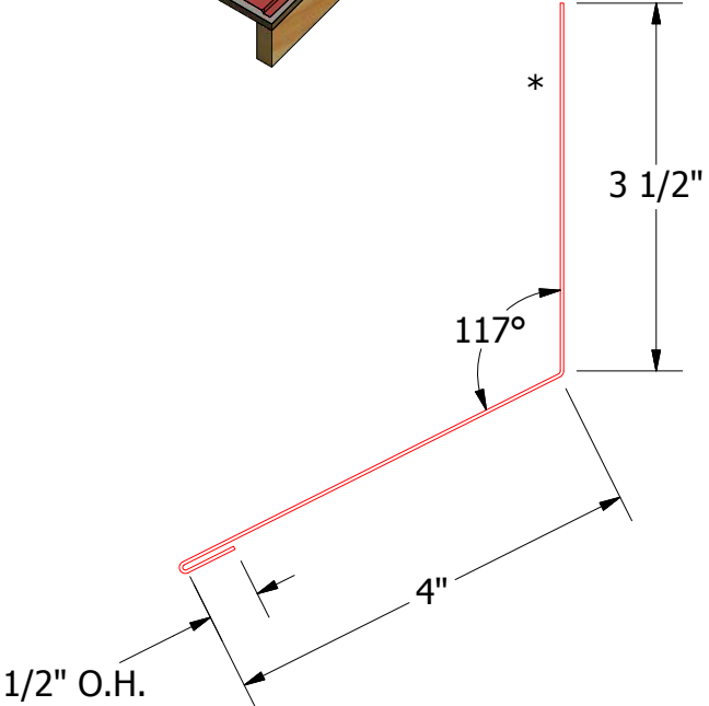
HSA500 - Headwall Trim
