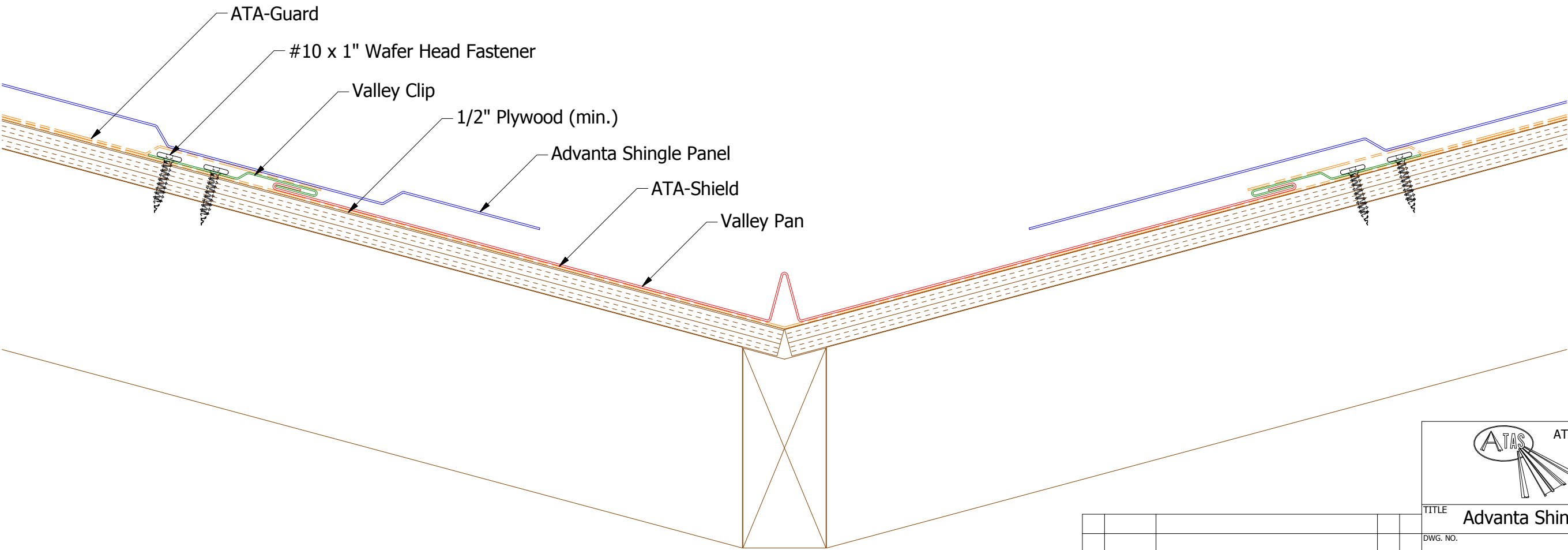
HSA806 - Valley Pan
