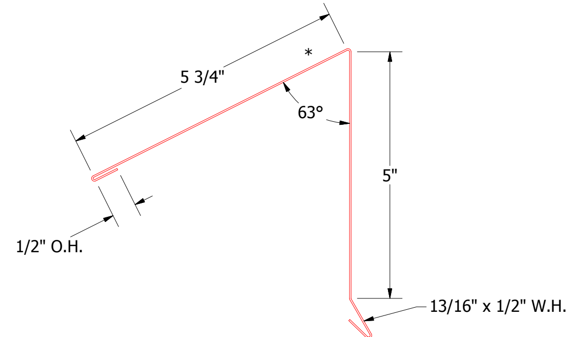
HSA342 - Shed Ridge Cap
