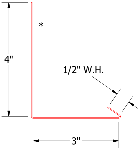
HSA440 - Step Flashing
