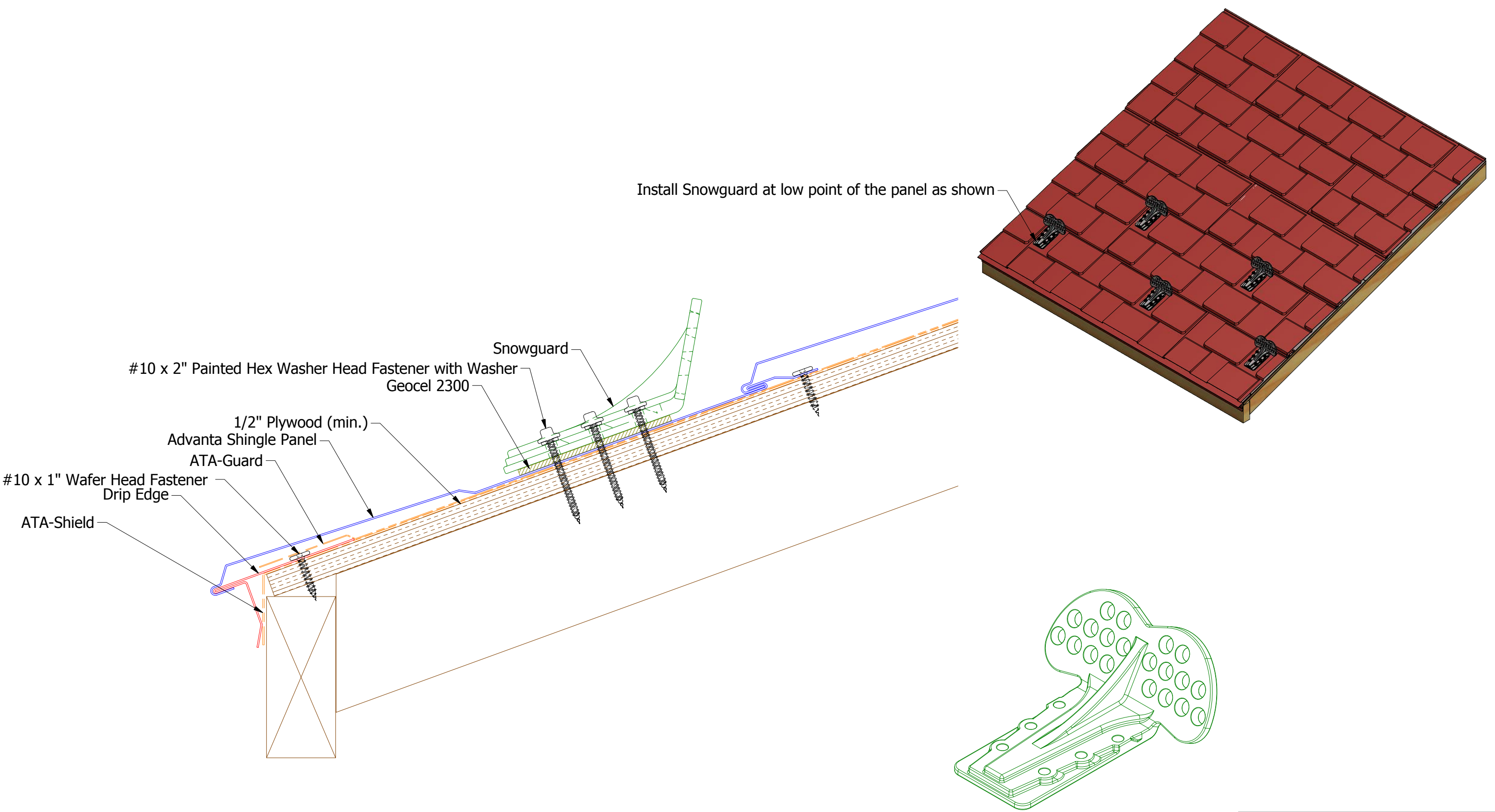
Snowguard
