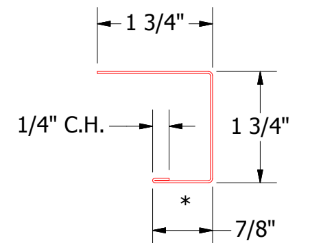
J Channel
