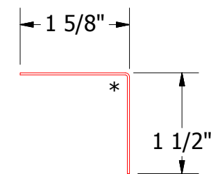
Angle Trim
