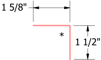
BWR680-Angle Trim
