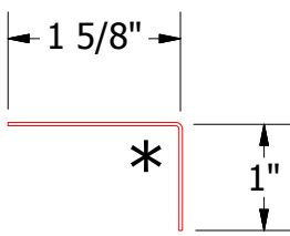
BCA680-Angle Trim
