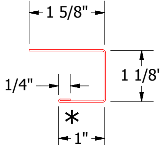
BCA118-J Channel
