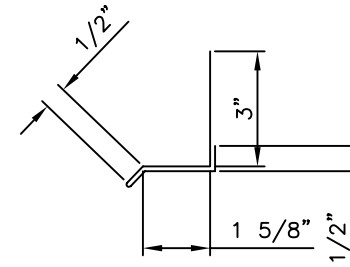
SILL TRIM
