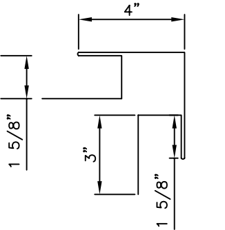
OUTSIDE CORNER TRIM
