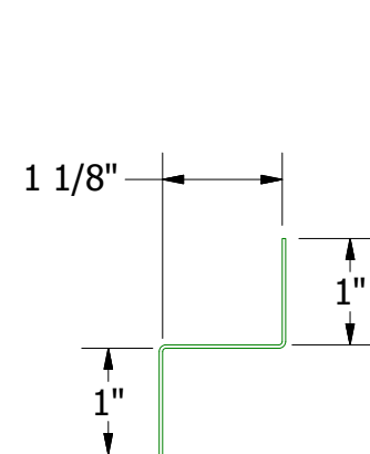
BPA681 - Support Z (if conditions apply)
