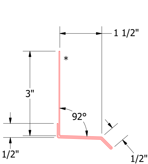
BPA661 - Base Trim
