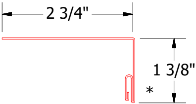
BPA139 - Snap Base
