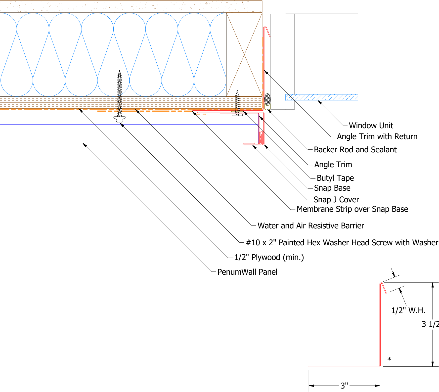
BPA683 - Angle Trim with Return
