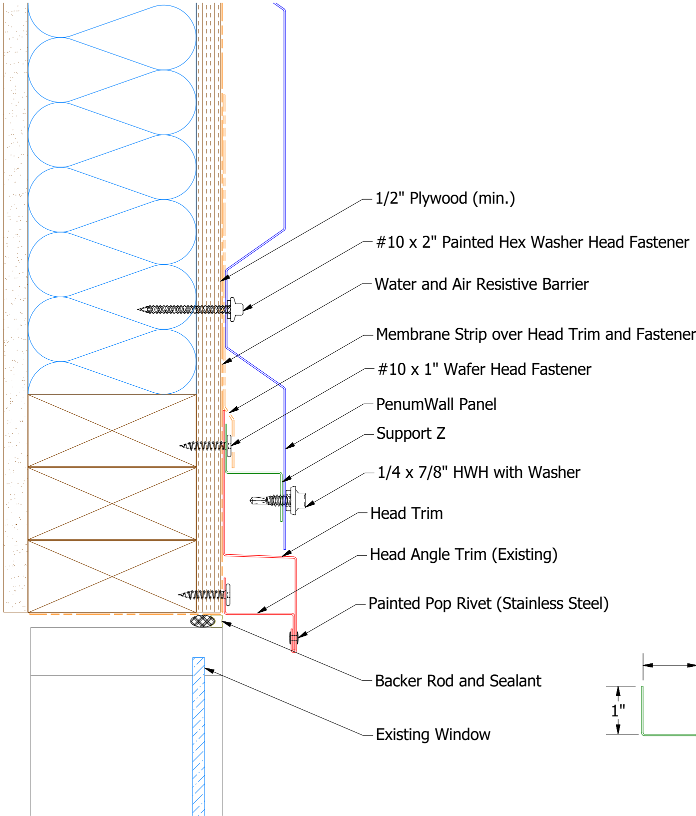
BPA681 - Support Z (if conditions apply)
