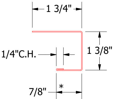
BPA138 - J Channel
