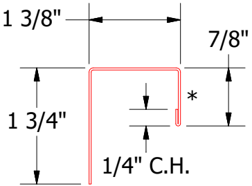
BPA158 - J Channel
