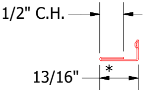
UNS078 - Snap J Cover
