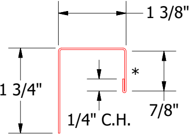
BPA158 - J Channel
