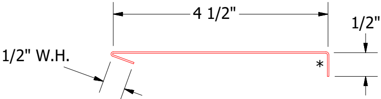
BPA690 - Head Angle Trim
