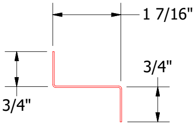
BPA691 - Head Angle Trim (Existing)
