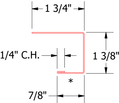
BPA158 - J Channel
