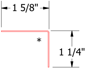
BPA680 - Angle Trim
