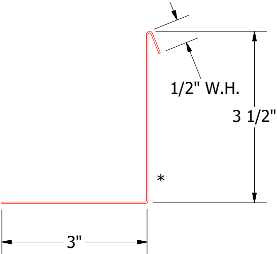
BPA683 - Angle Trim with Return
