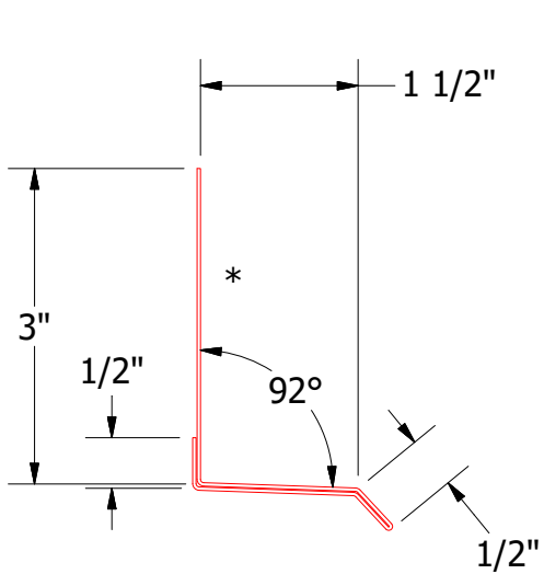
BPA661 - Base Trim
