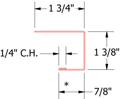
BPA138 - J Channel
