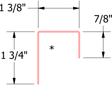
BWA270 - J Closure
