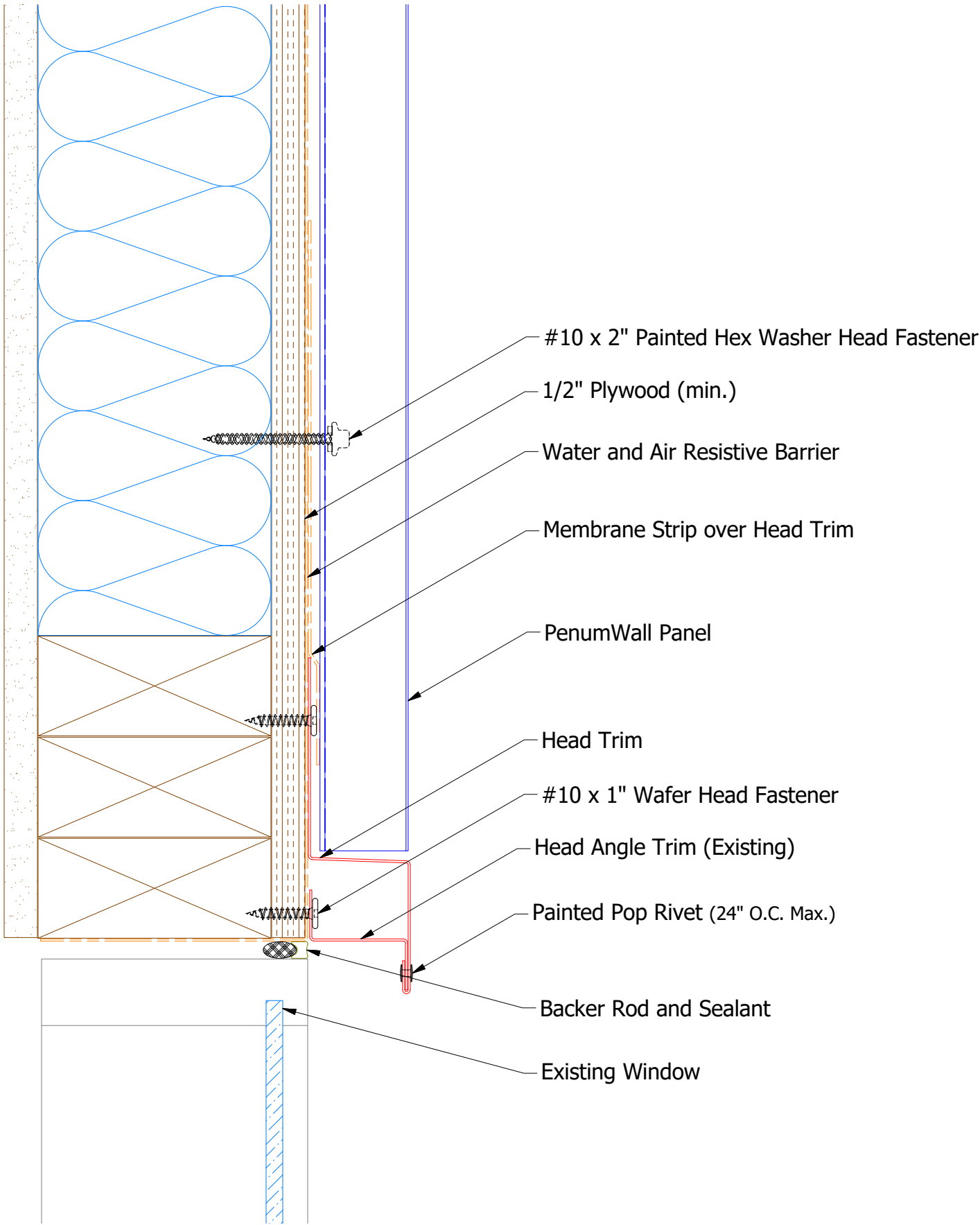
BPA550 - Head Trim
