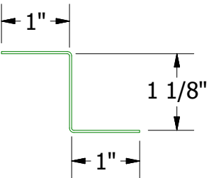
BPA681 - Support Z (if conditions apply)
