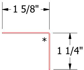
BPA680 - Angle Trim
