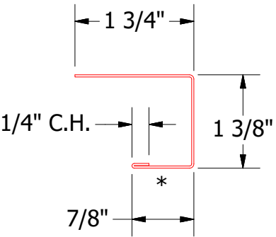
BPA158 - J Channel
