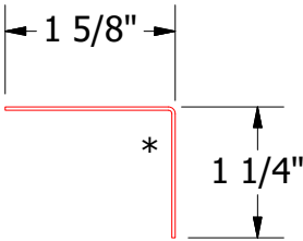
BPA680 - Angle Trim
