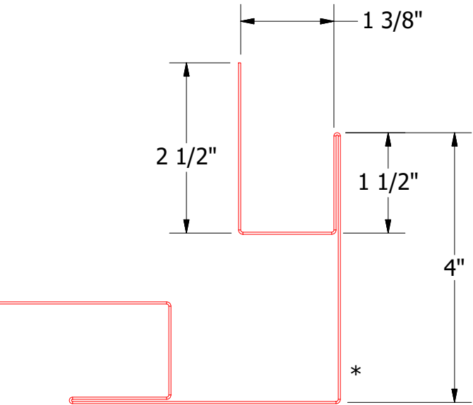
BPA602 - Outside Corner Post
