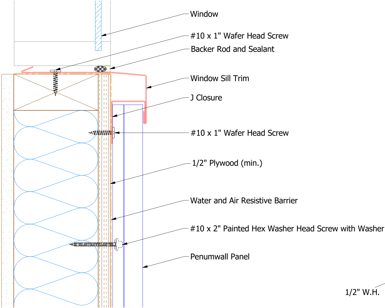
BPA670 - Window Sill Trim
