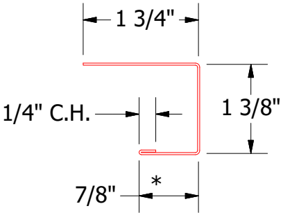
BPA138 - J Channel
