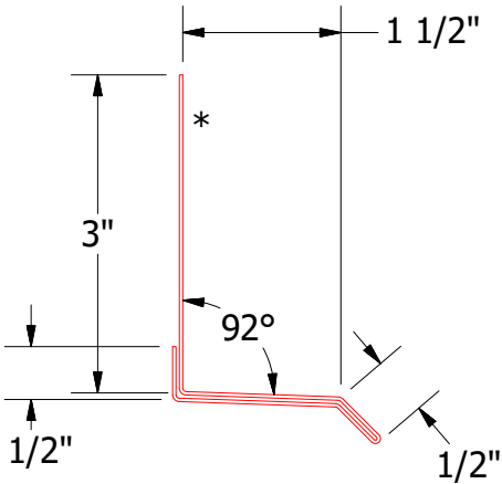
BPA661 - Base Trim
