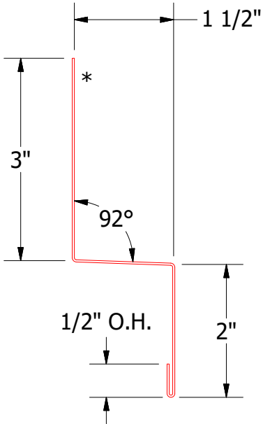
BPA550 - Head Trim
