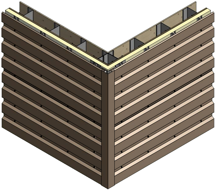
BPA602-Outside Corner Post
