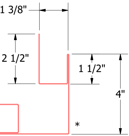
BPA602-Outside Corner Post
