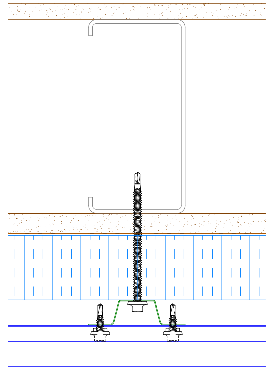
Alternate Subgirt Orientation (NTS)
