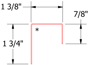
BPA270-J Closure
