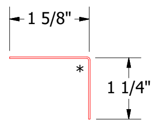
BPA280-Angle Trim
