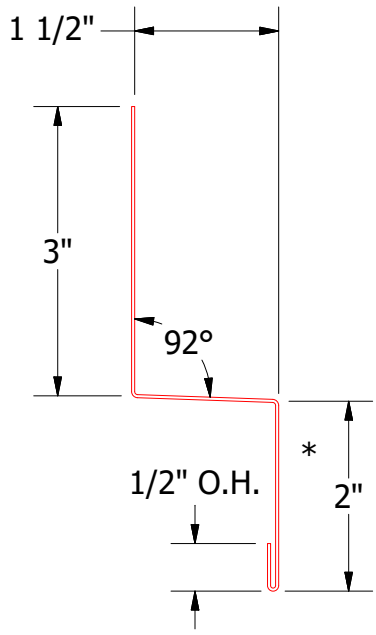
BPA550-Head Trim
