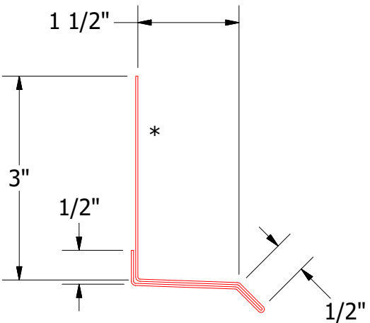
BPA661-Base Trim
