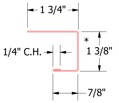
BPA138-J Channel
