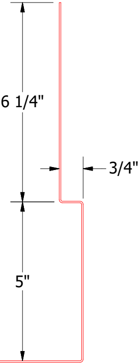
Support Plate
