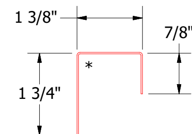
BPA270-J Closure
