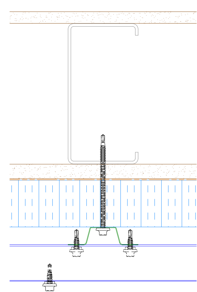
Alternative Subgirt Orientation (NTS)
