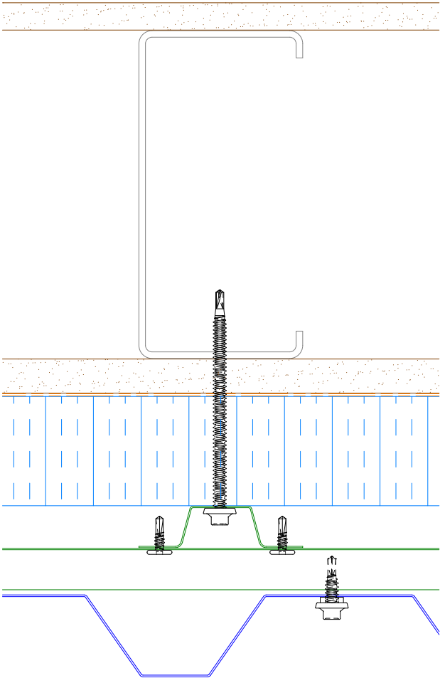
Alternative Subgirt Orientation (NTS)
