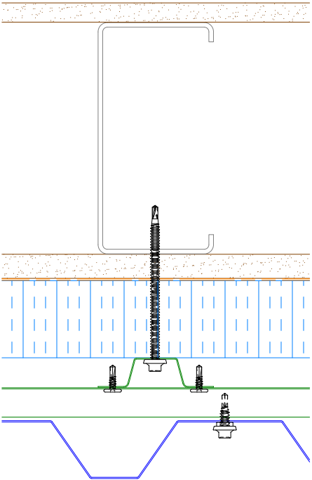
Alternate Subgirt Orientation
