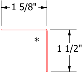
BWA680-Angle Trim
