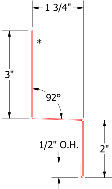
BWA550-Head Trim
