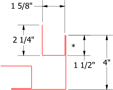
BWA602-Outside Corner Post
