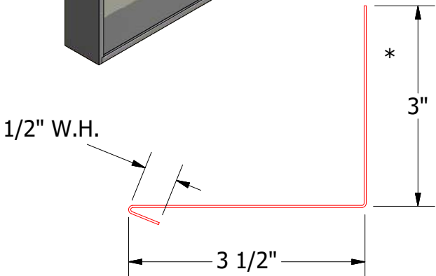
BWA683-Angle Trim with Return (Field Fabricated from Color Matched Flat Stock)
