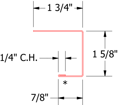
BWA158-J Channel
