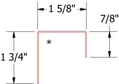
BWA270-J Closure
