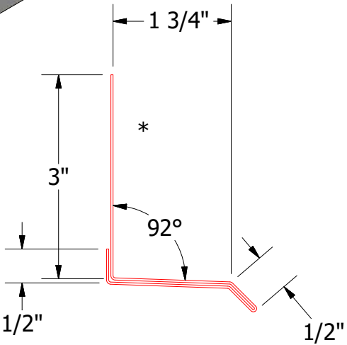
BWA661-Base Trim
