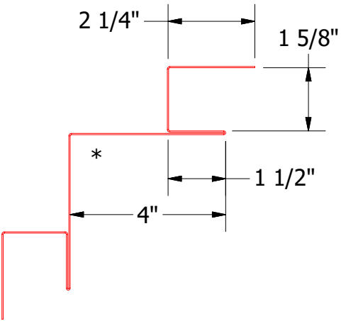
BWA601-Inside Corner Post
