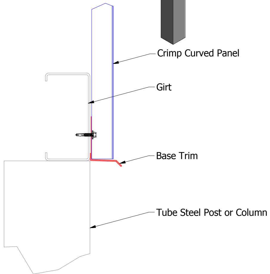
DETAIL A
