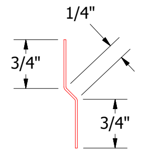
HCA975-Joggle Cleat
