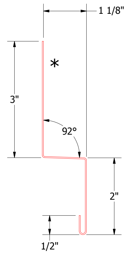
HCAXXX-Head Trim
