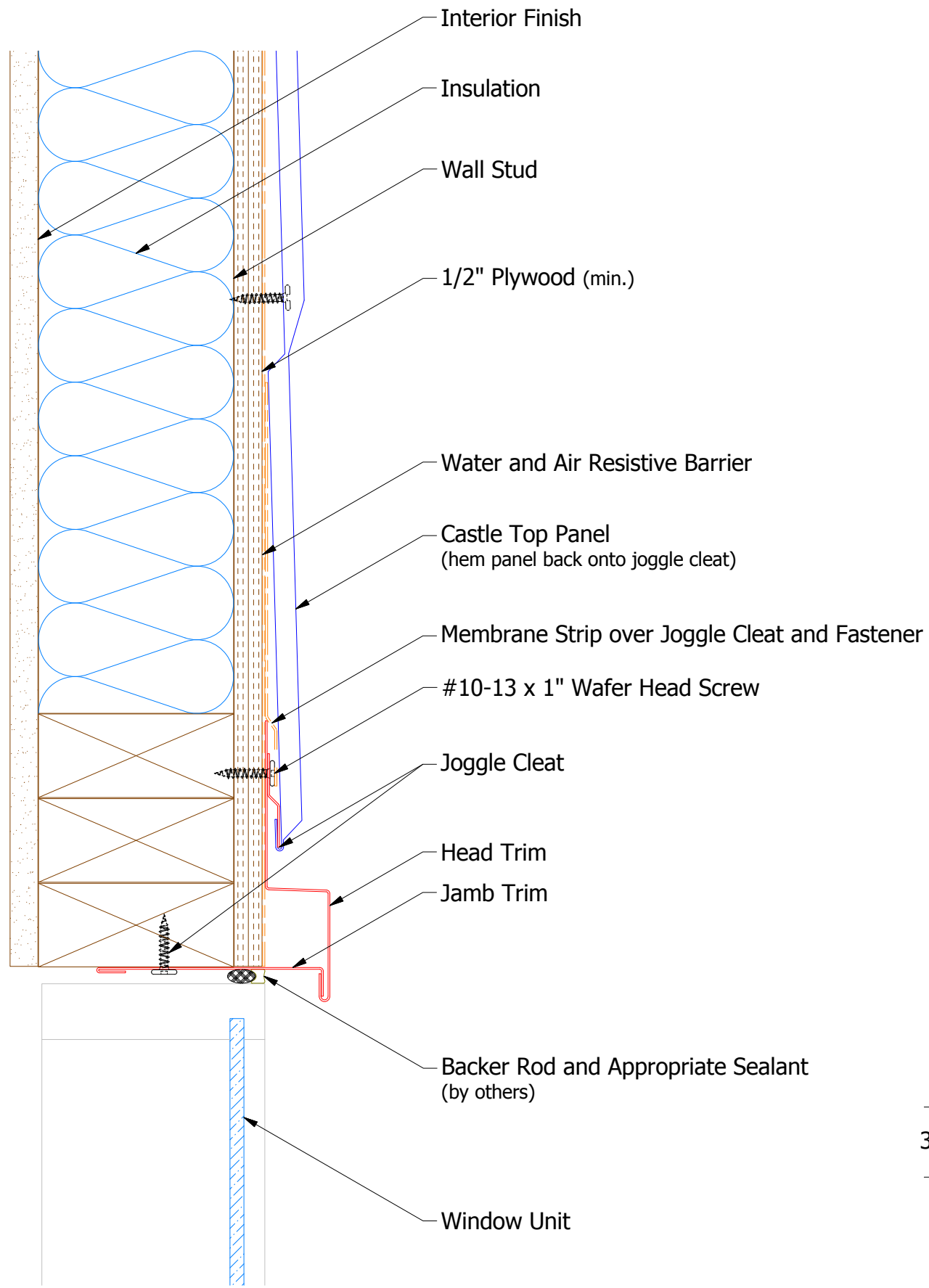
Wall Application
