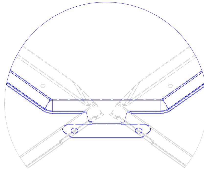
DETAIL B
