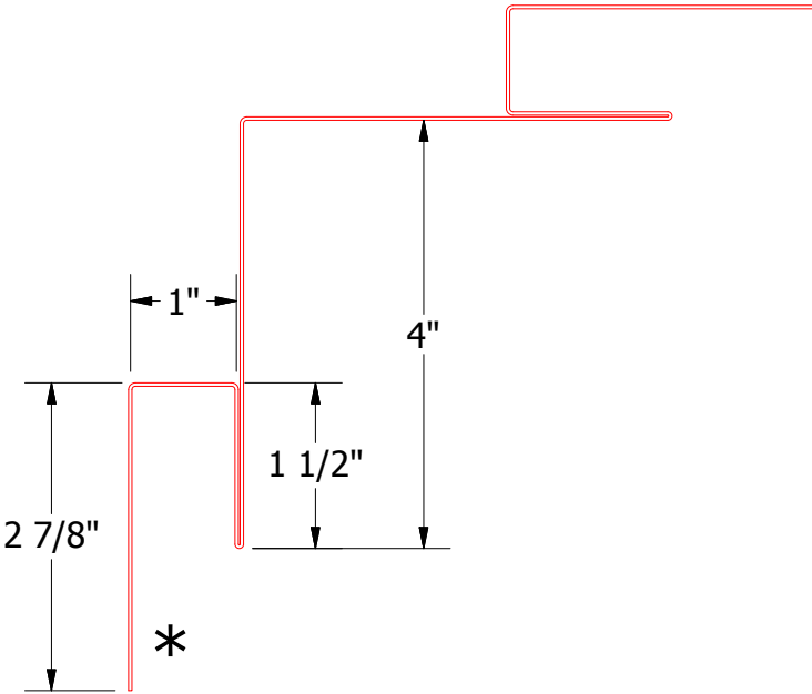
HCAXXX-Inside Corner Post
