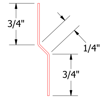
HCA975-Joggle Cleat
