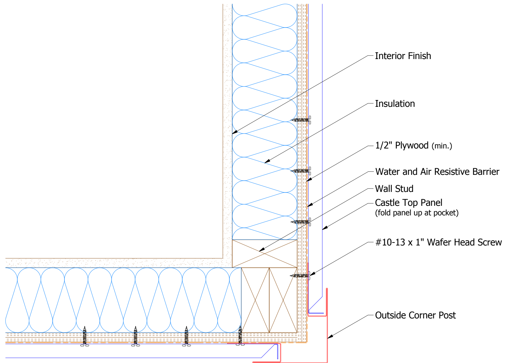
HCAXXX-Outside Corner Post
