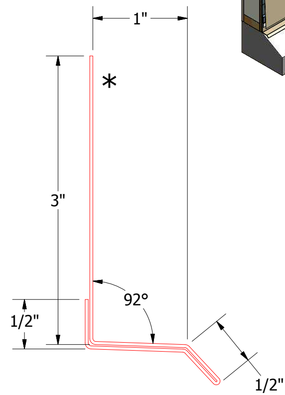
HCAXXX-Base Trim
