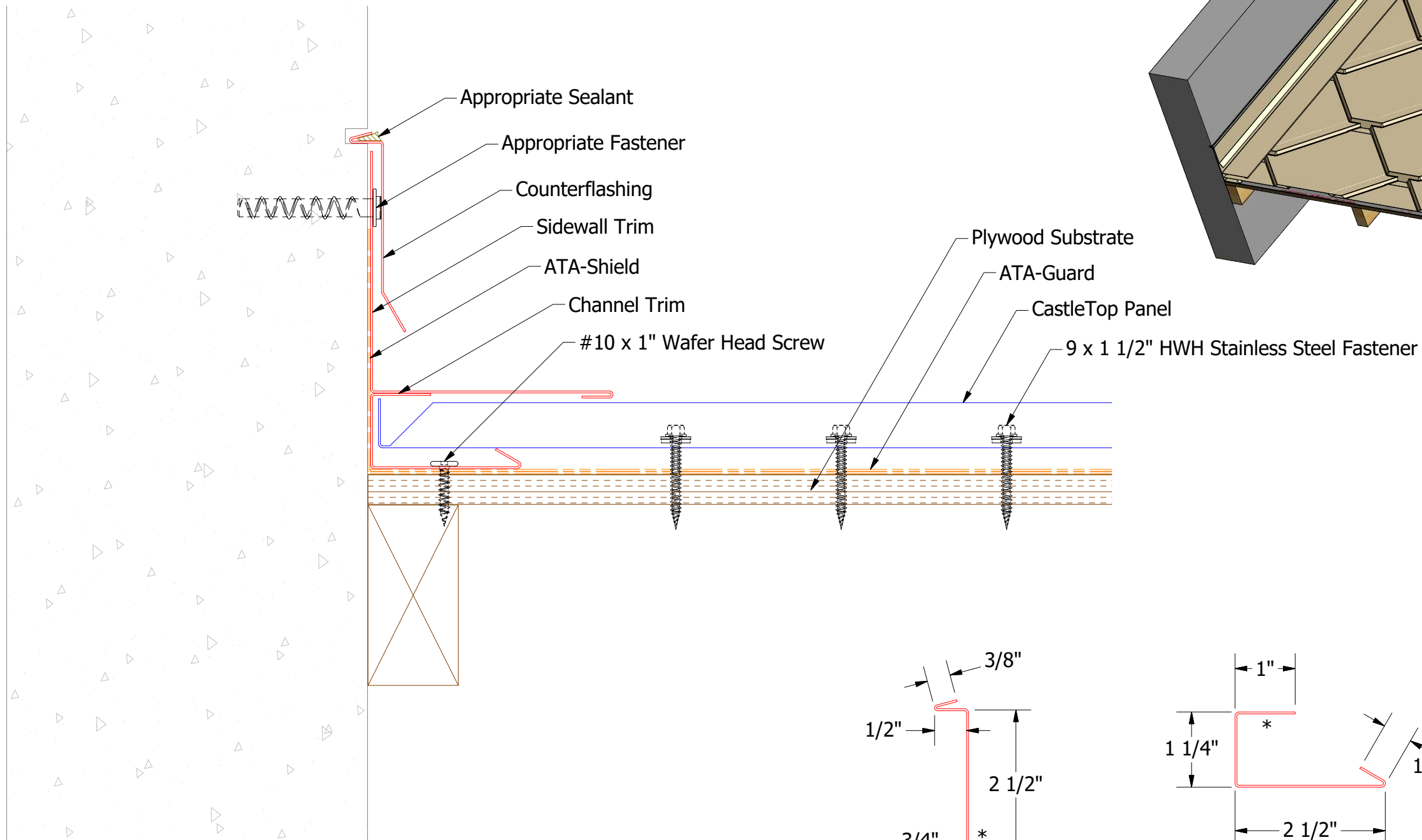
HCA200 - Channel Trim
