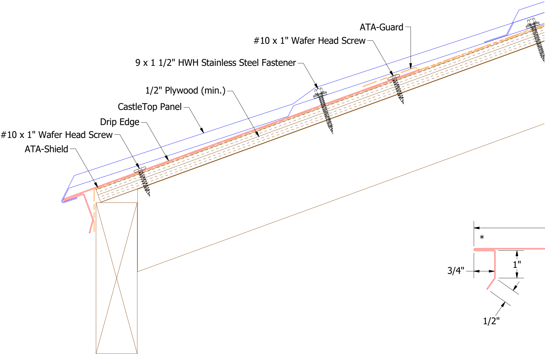
Install Drip Edge Fasteners so CastleTop Panels will conceal them
