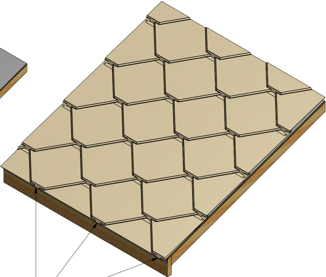
Fold CastleTop Tabs around Drip Edge Trim
