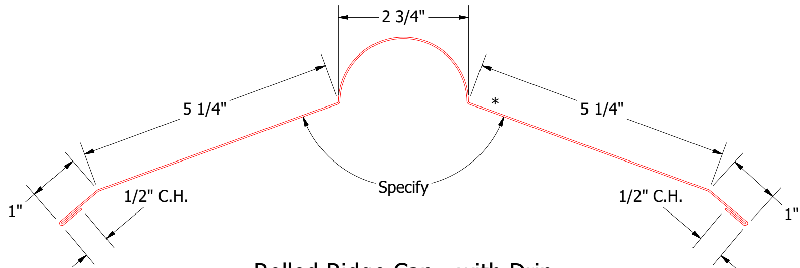
Rolled Ridge Cap - with Drip
