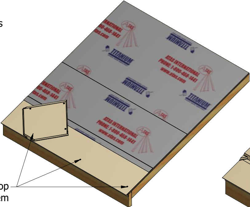
Bearing Plate used at Eave in High Wind Applications
