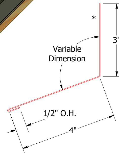
HLA500-Headwall Trim
