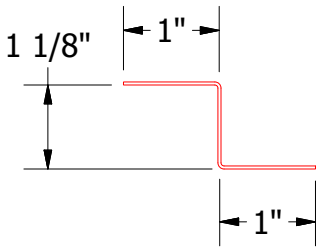
HLA910-Z Closure
