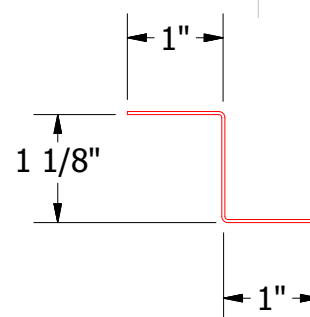
HLA910-Z Closure
