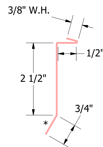
HLA980-Counterflashing
