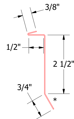
HLA980-Counterflashing
