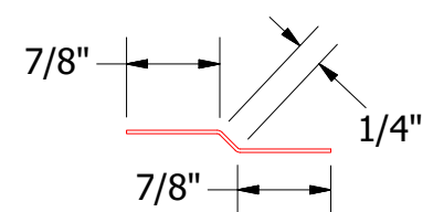
HLA975-Joggle Cleat
