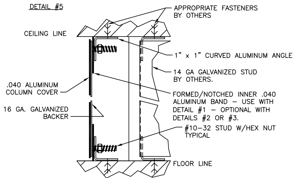
TOP & BOTTOM COLUMN COVER CONNECTION FOR VERTICAL REVEAL JOINTURES
