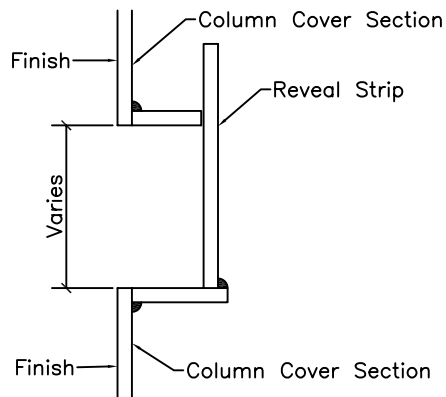
Offset Reveal
