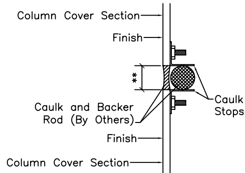
Caulk Joint Reveal
