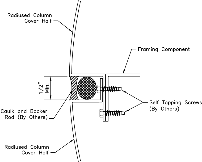
Caulk Joint Reveal
