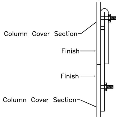
Hairline Reveal
