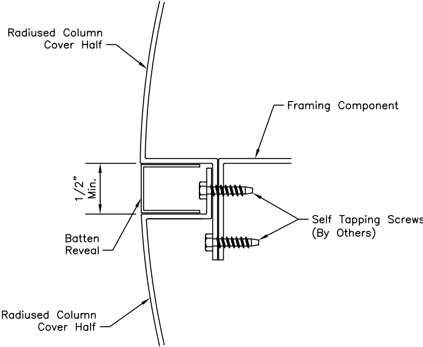
Batten Reveal
