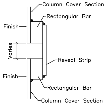
Standard Offset Reveal
