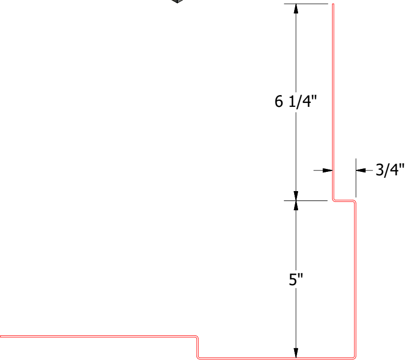
Support Plate
