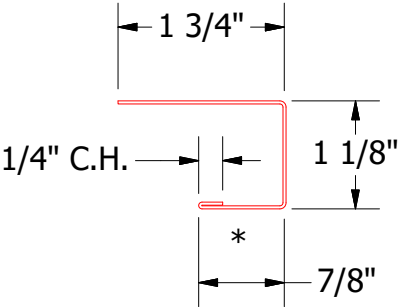
MCA118-J Channel
