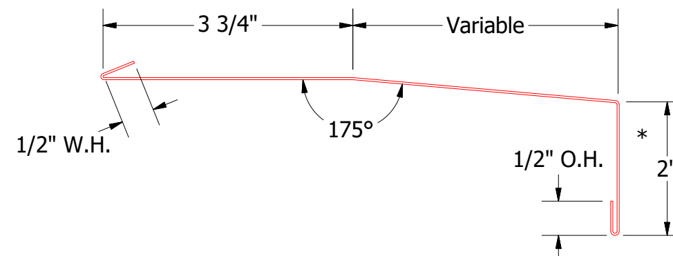
MCA670-Window Sill Trim
