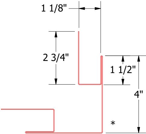
MCA602-Outside Corner Post
