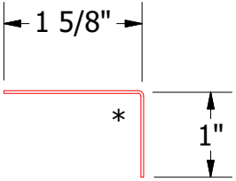
MCA680-Angle Trim
