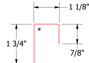
MCA270-J Closure
