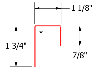
MCA270-J Closure
