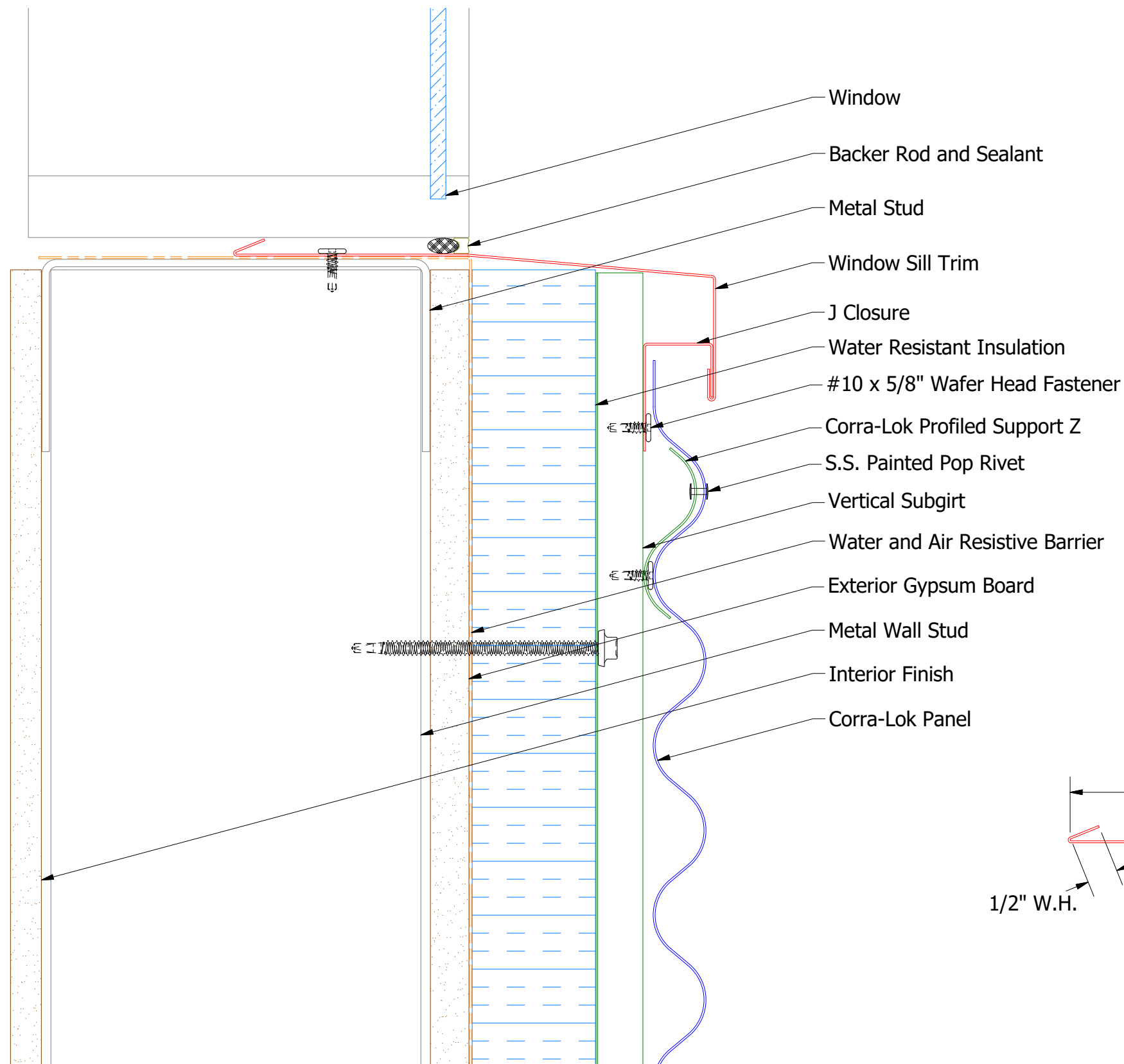
MCA682 Corra-Lok Profiled Support Z
