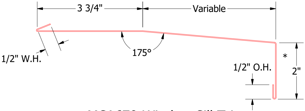
MCA670-Window Sill Trim
