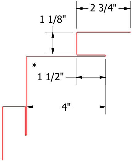
MCA601-Inside Corner Post
