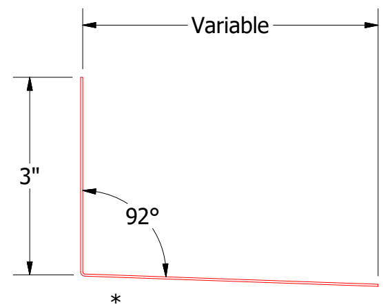
Flashings (Field Fabricated From Color Matched Flat Stock)
