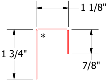
MCA270-J Closure
