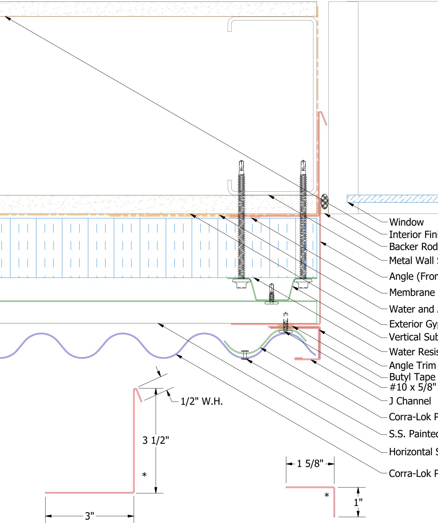
MCA683-Angle Trim with Return
