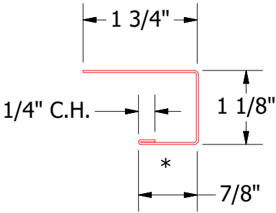
MCA118-J Channel
