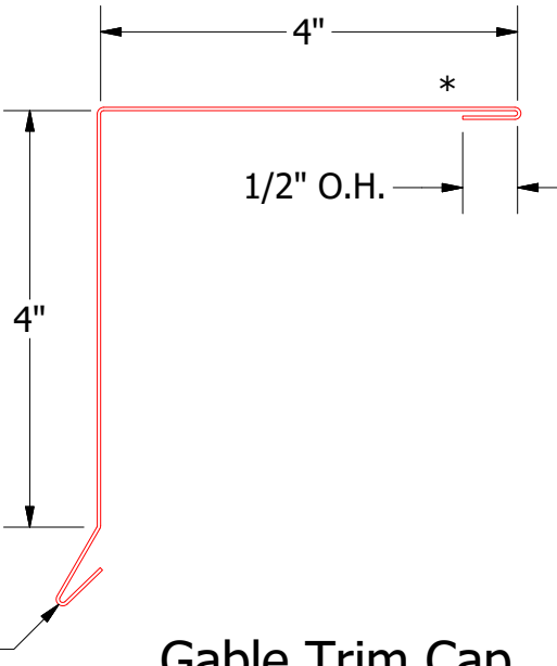
Gable Trim Cap
