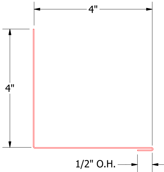
Sidewall Trim
