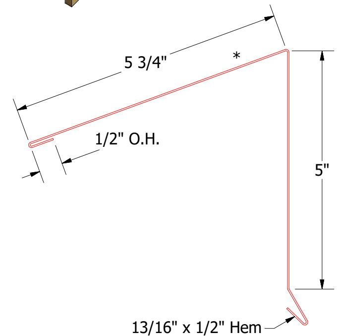
Shed Ridge Cap
