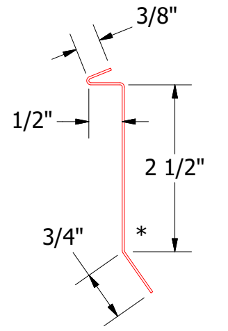
Counterflashing
