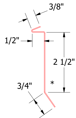
Counterflashing
