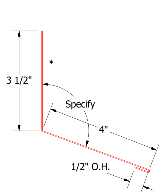
Headwall Trim
