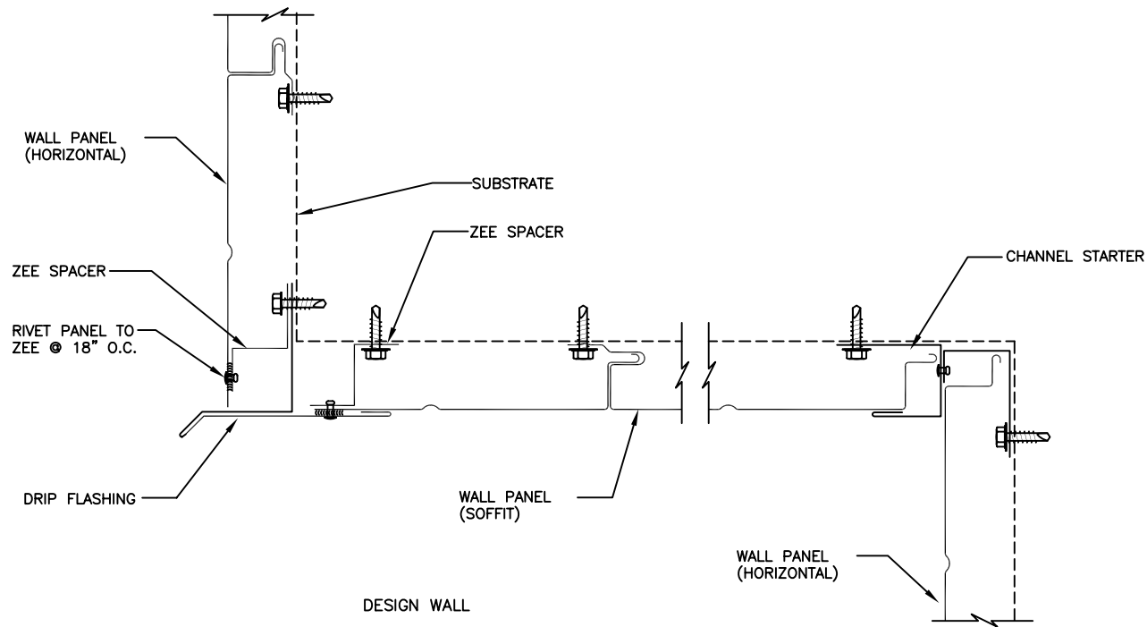
SOFFIT TO WALL DETAIL
