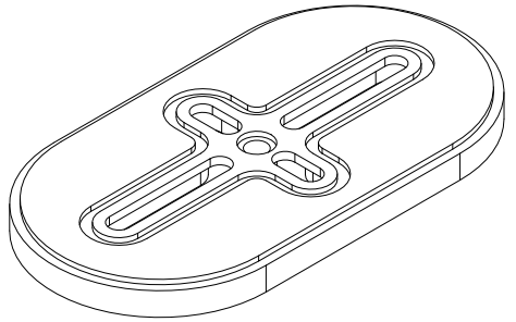
ASV Shim
