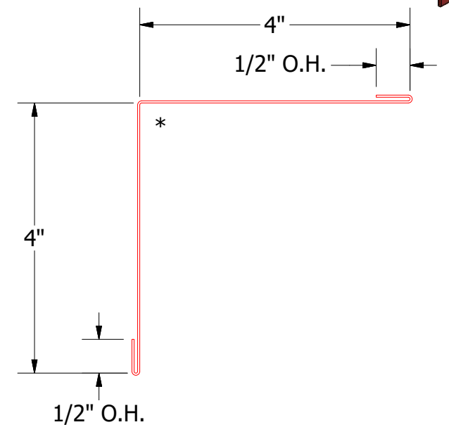
MDA600 - Inside Corner Cap
