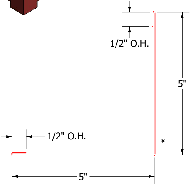
MDA610 - Outside Corner Cap
