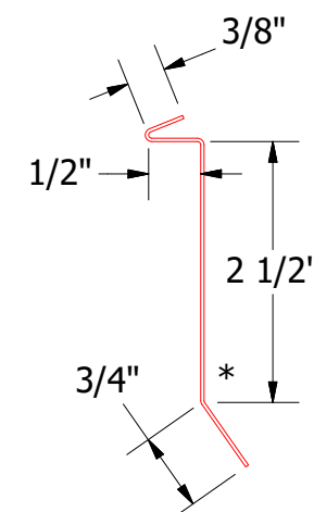
MDA980 - Counterflashing
