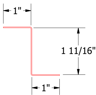
MDA910-Z Closure
