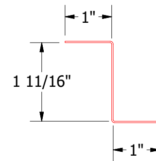
MDA910 - Z Closure
