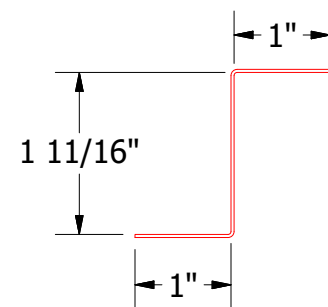
MDA910 - Z Closure
