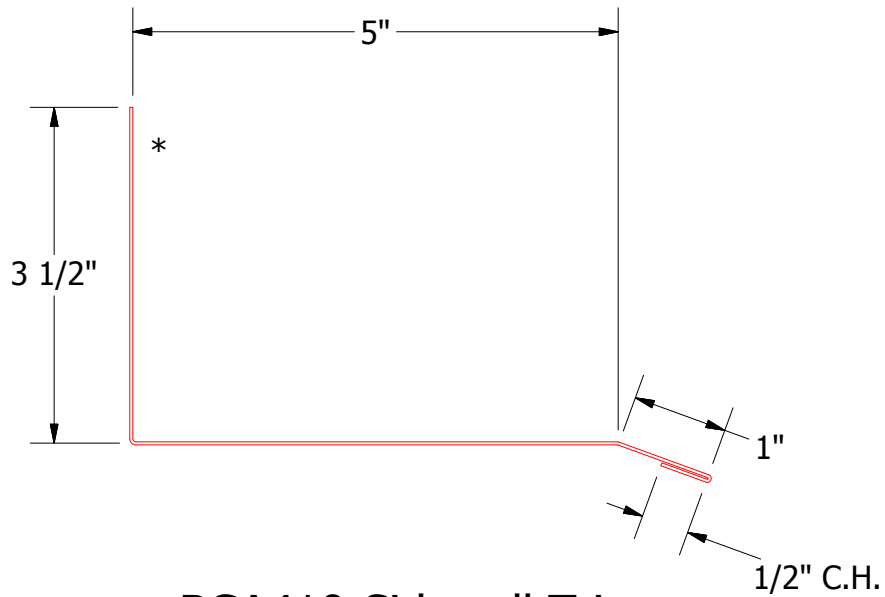
BGA410-Sidewall Trim
