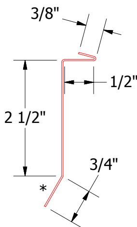
BGA980-Counterflashing
