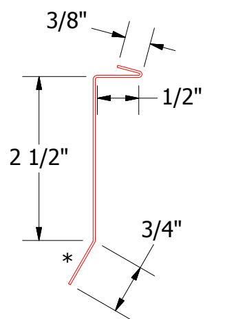
BGA980-Counterflashing
