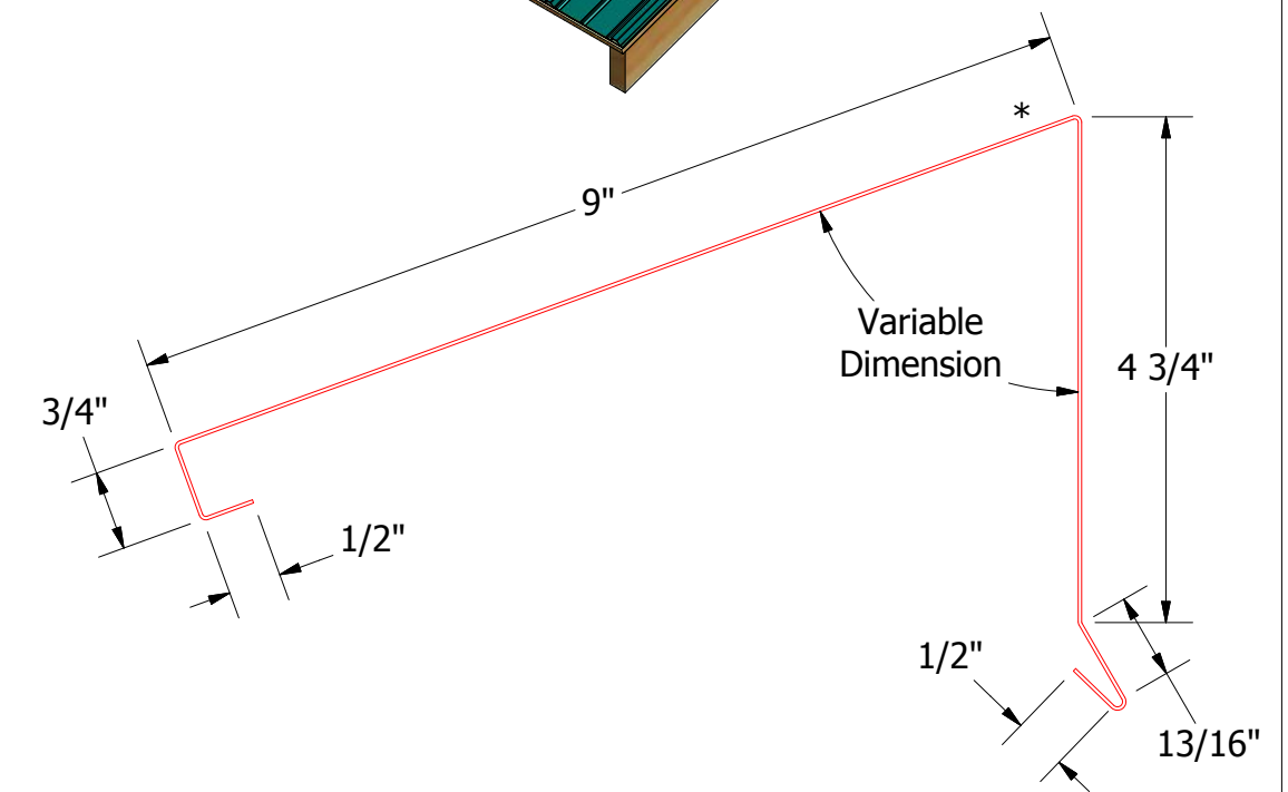
BGA366-Vented Shed Ridge Cap
