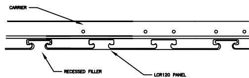
LINEAR CEILING - Recessed Filler
