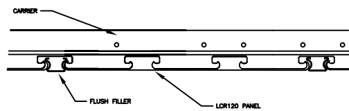
LINEAR CEILING - Flush Filler
